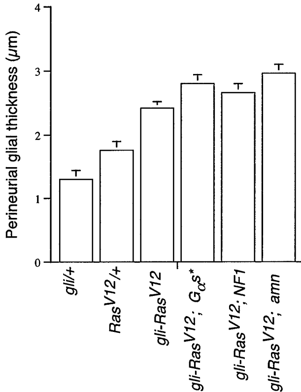
Figure 2: Enhancement of the effects of a strong Ras^{V12} by overexpression of amn , NF1 and G_{\alpha S}
