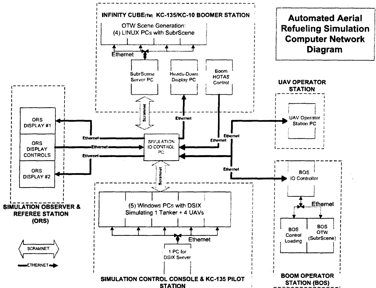
Figure 1. AAR Simulation Environment Structure.
