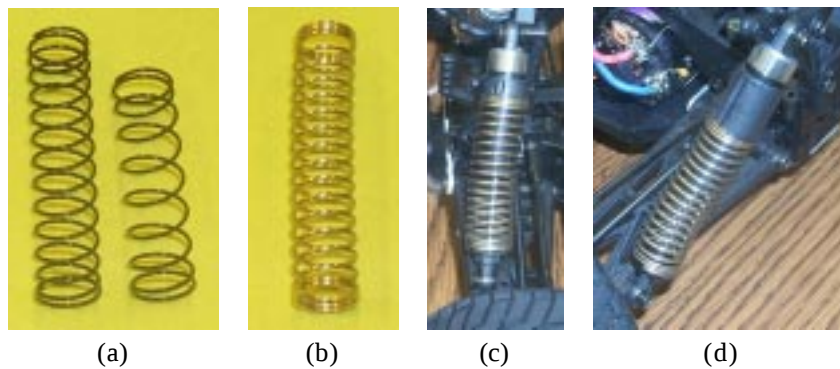
Figure 3: (a) The original springs that came with the HPI chassis. (b) The spring used to stiffen the suspension. (c) Detail of front shock absorbers and (d) rear shock absorbers.
