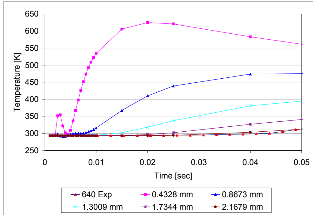
Figure 12. Sub-surface model prediction at 640 mm from the RFT showing the perturbation that occurs near the ID.
