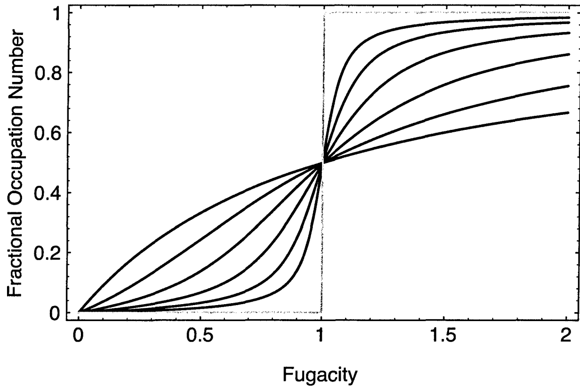
Figure 1: f_L(z) versus z for several values of L . The black curves represent L values from 1 to 6, with increasing steepness, while the gray curve is the limit as L \rightarrow \infty .
