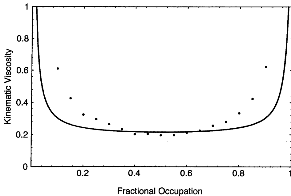
Figure 6: Viscosity versus f for L = 2 .
