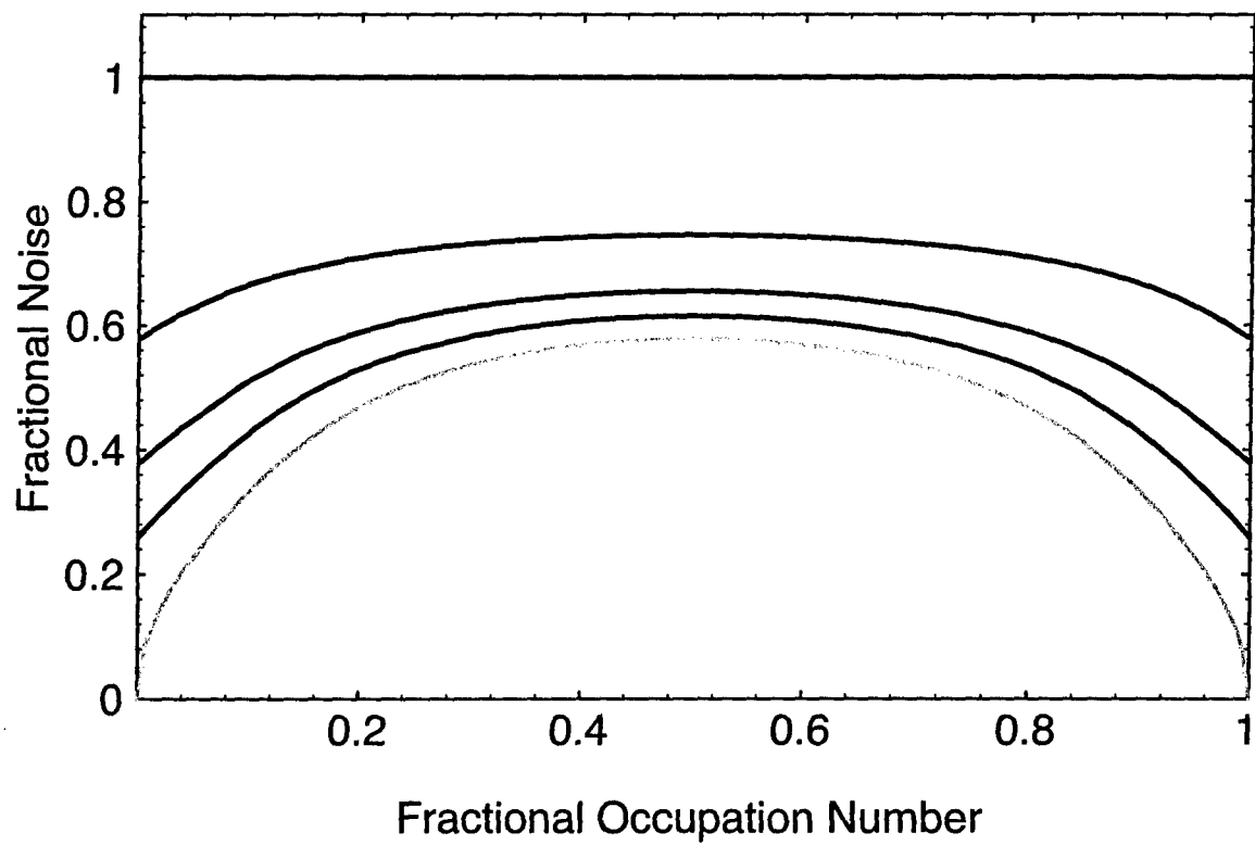
Figure 7: \Delta\mathcal{F}_L versus f for several values of L . The black curves represent L values from 1 to 4, increasing downward, while the gray curve is the limit as L \rightarrow \infty .
