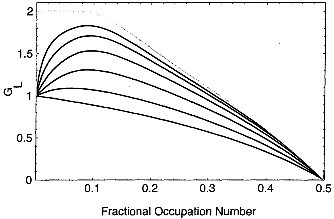
Figure 3: G_L versus f for several values of L . The black curves represent L values from 1 to 6, increasing upward, while the gray curve is the limit as L \rightarrow \infty .
