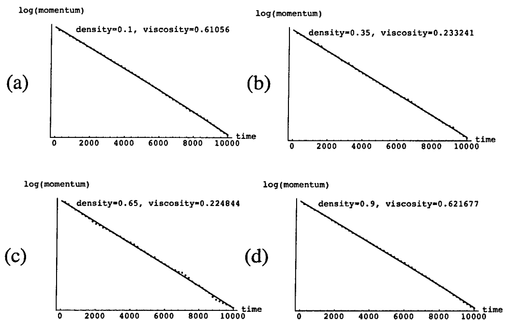
Figure 5: Time decay of shear-wave amplitude
