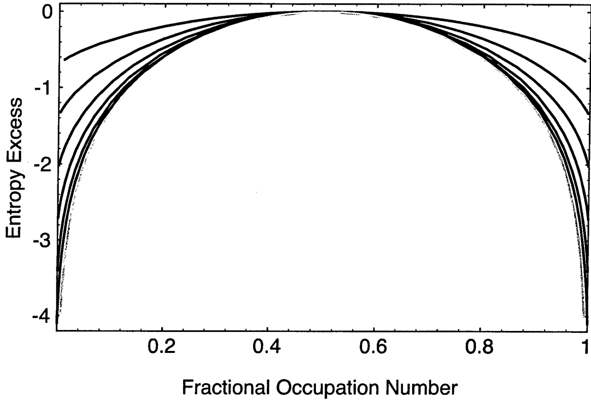
Figure 2: Entropy excess \Delta S_L versus fractional occupation number f_L(z) . The black curves represent L values from 1 to 6, increasing downward, while the gray curve is the limit as L \rightarrow \infty .
