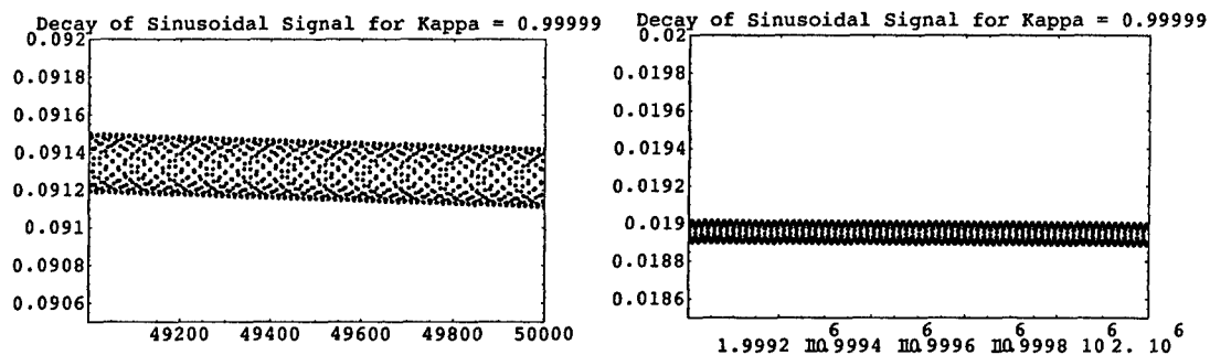
Figure 8: Decay of sinusoidal density profile for \kappa = 0.99999
