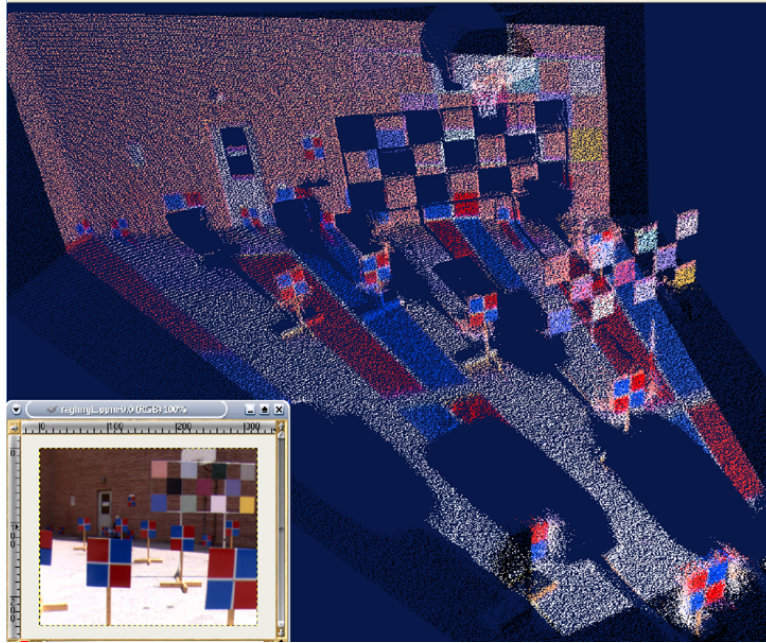
Figure 5. Visualization of registration of Riegl sensor data to color camera image at lower left. (The colors of the 3-D foreground posters match the image, as do un-occluded elements of the background [the door, for example], indicating a good registration.)
