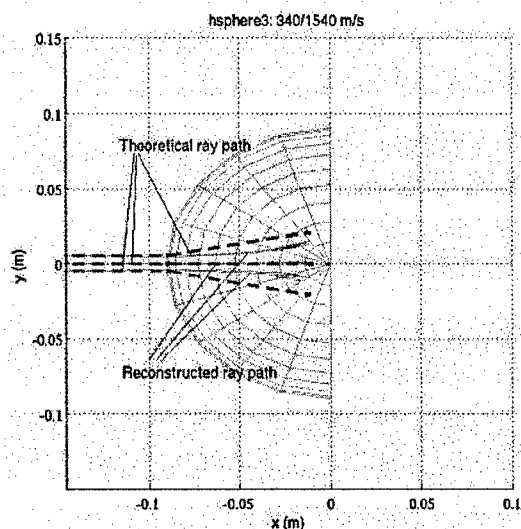
Fig 22: Ray path for the hemisphere model.
