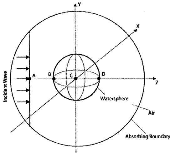
Fig 11: The 3D water sphere FEA model.
