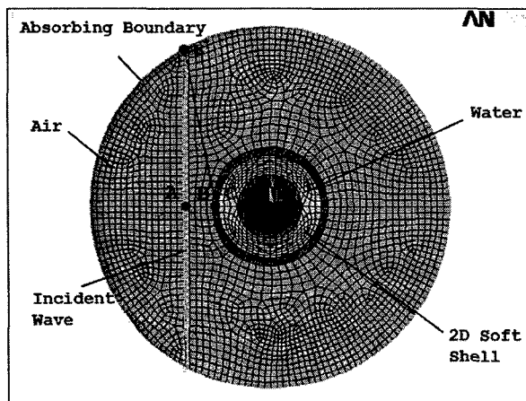
Fig 8: The soft shell 2D FEA model generated in ANSYS.
