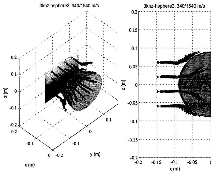
Fig 21: Ray paths calculated based on FEA data.
