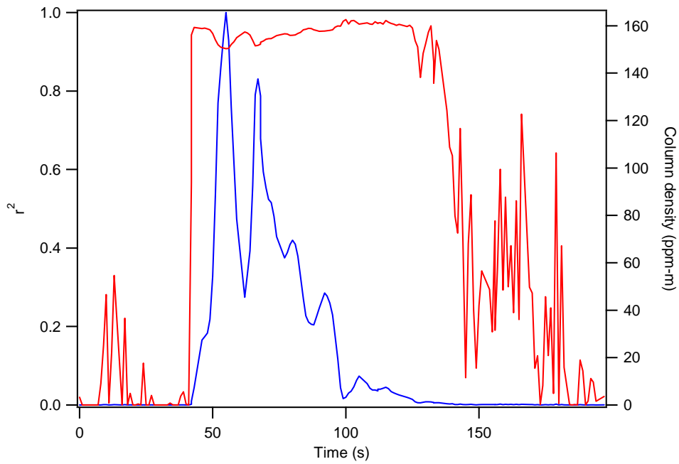
Figure 11. 3D Overlay plot of all radiance spectra ( \text{Watts/cm}^2\text{-sr-cm}^{-1} ) collected with CATSI sensor (top view), graph of the related CL (blue curve) and global r^2 (red curve) (lower graph) for a measurement performed on a plume generated with a flow rate of 100 L/min. Measurement performed at 16h17 (CATSI time) on absorbent background.
