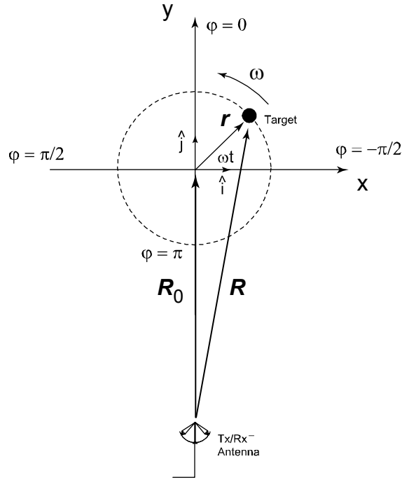
Figure 28. Configuration for measurement of oscillatory target motion. ( \omega = 1.2 \text{ rpm} )
