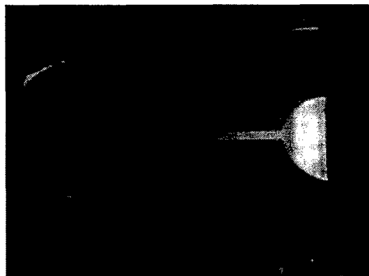
Figure 15. Photographs of pulsed discharges in M=4 flows at P_0=760 torr, P_{\text{test}}=10 torr, pulse repetition rate 40 kHz. Left: nitrogen, B=0 ; right: air, B=1.5 T. The discharge is seen at an oblique angle, looking in the direction of the flow.
