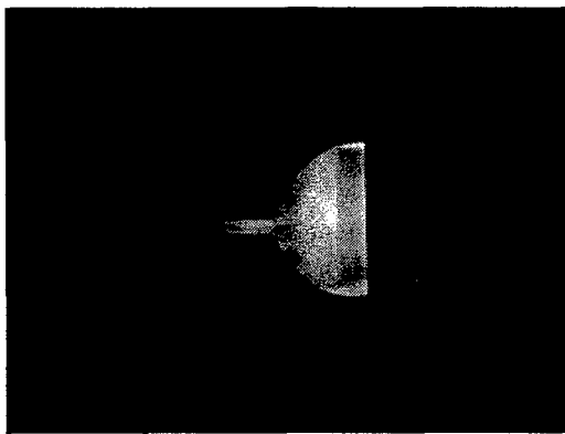
Figure 15. Photographs of pulsed discharges in M=4 flows at P_0=760 torr, P_{\text{test}}=10 torr, pulse repetition rate 40 kHz. Left: nitrogen, B=0 ; right: air, B=1.5 T. The discharge is seen at an oblique angle, looking in the direction of the flow.
