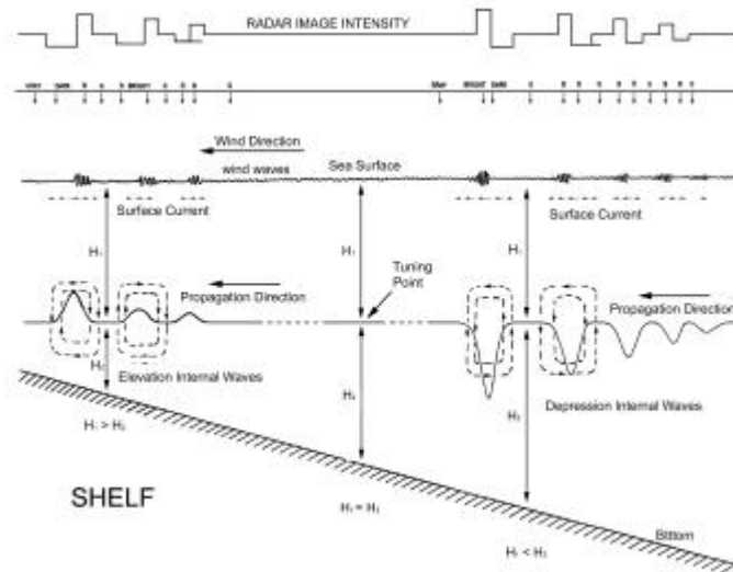
Figure 3. Schematic diagram of depression and elevation internal waves, surface current field, wind waves, and the resultant SAR image intensity variations. (After Liu, et al., 1998).
