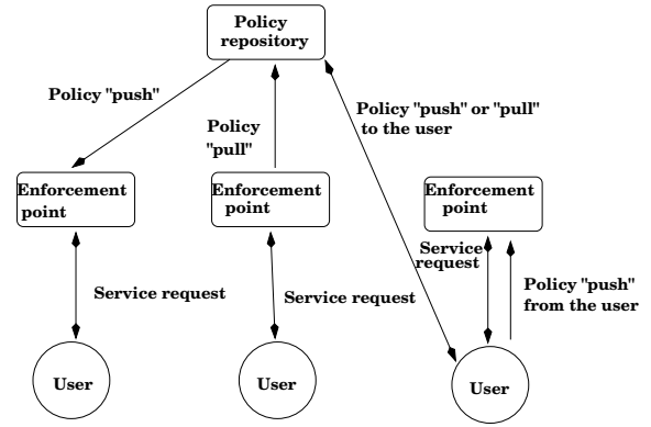
Figure 6: Policy distribution models.
