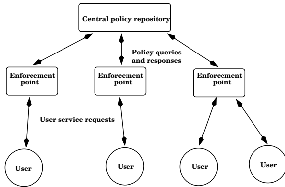
Figure 3: Centralized policy specification and enforcement.
