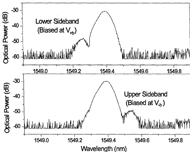
Fig. 6. Measured optical output SSB spectrums on OSA at a modulation frequency of 18 GHz.
