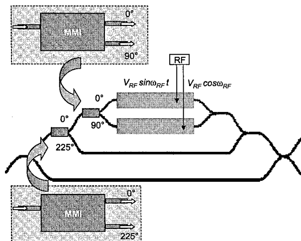
Fig. 12. The realization of the new generation of phase shifter structure incorporating MMI couplers.
