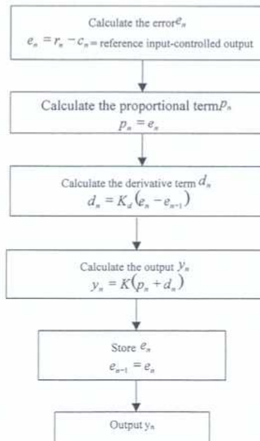
Fig. 2-6. Flowchart of the PD controller
