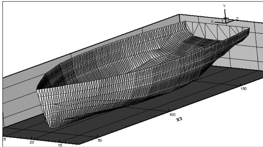
Figure 6: TNT Explosion Beneath Ship Hull with 3D AGS (X-Z Scales are not Proportional)
