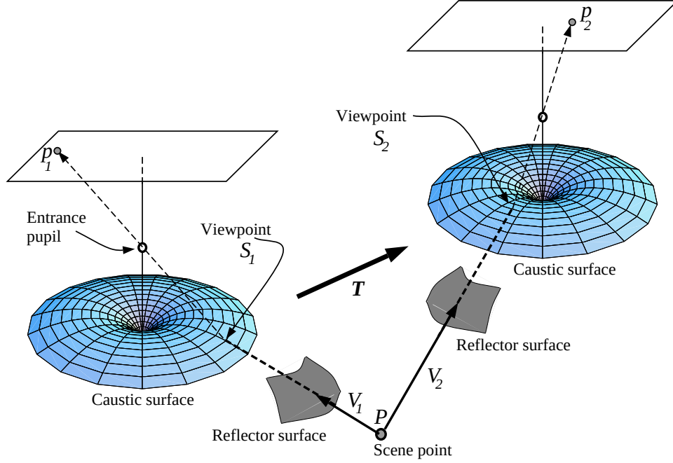
Figure 16: The catadioptric imaging system is represented here by only its caustic surface (viewpoint locus). The two caustic surfaces denote the same camera after being given a known translation \mathbf{T} . An unknown scene point P visible from both views gets imaged at two point p_1 and p_2 respectively. From the caustic model and the hypothesized parameters during search, we map these image point to their respective viewpoint S_1 and S_2 and their viewing directions V_1 and V_2 . When the right model parameters are estimated, the two position vectors (light rays at viewpoints) must meet at the scene point.
