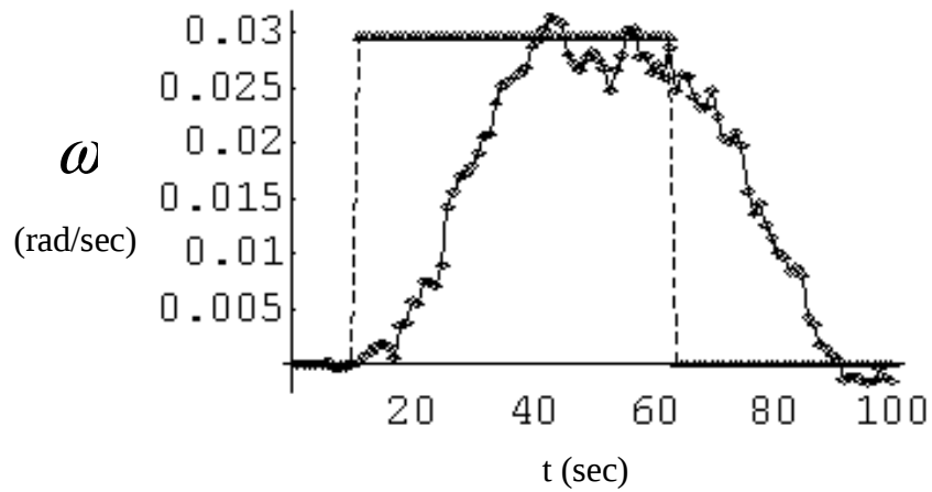
Figure 2 - IMMKE Turn Rate Estimate Turn rate (dashed) and turn rate estimate for target 4 averaged over 10 scenario runs.
