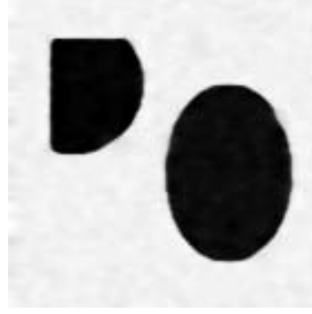
TV restoration and inpainting
