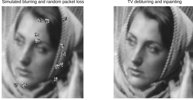
Figure 1: TV Inpainting of a blurred image (by K_1 in (13)) with simulated random packet loss.
