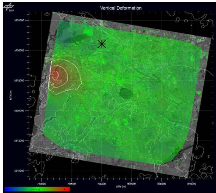
Fig.18 Ground inflation due to ground water regulation at the Berlin Olympic stadium. PS measurements have been spatially interpolated to allow for a better visual interpretation (green: no subsidence/inflation, red: inflation of 4 mm/year, cross: reference point, assumed to be stable; (Kampes et al., 2003).
