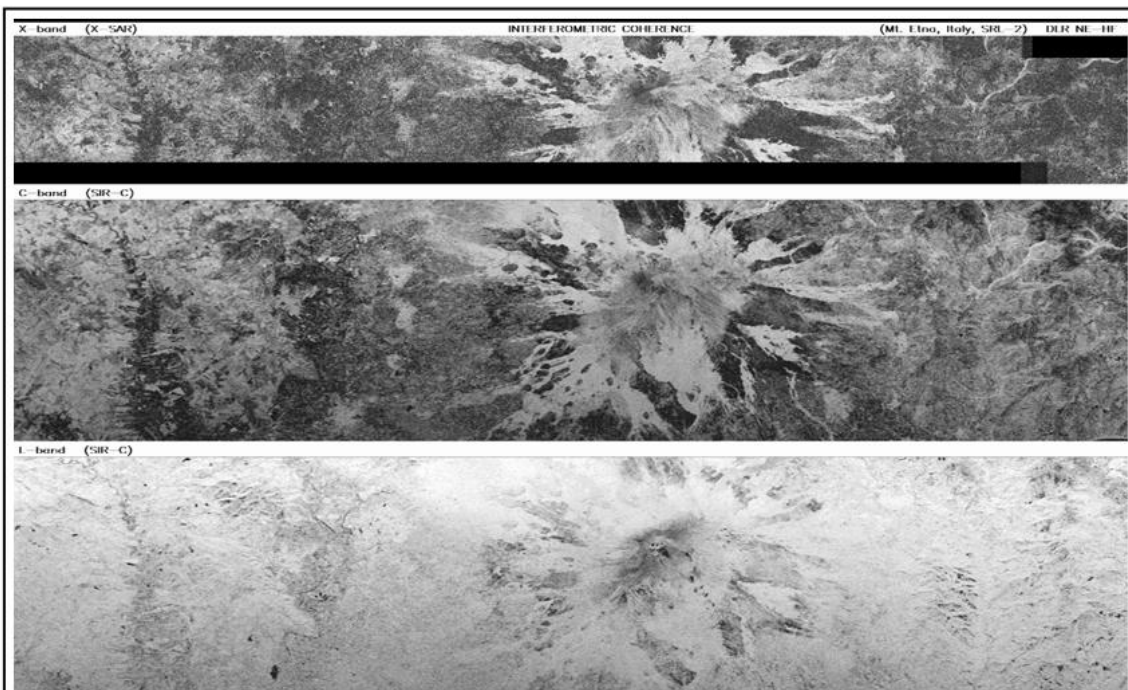
Fig21 Set of co-registered slant range coherence images in L-, C-, and X-band. White indicates high coherence and black low coherence. It is evident that L-Band has a high coherence with the exception of certain small areas
