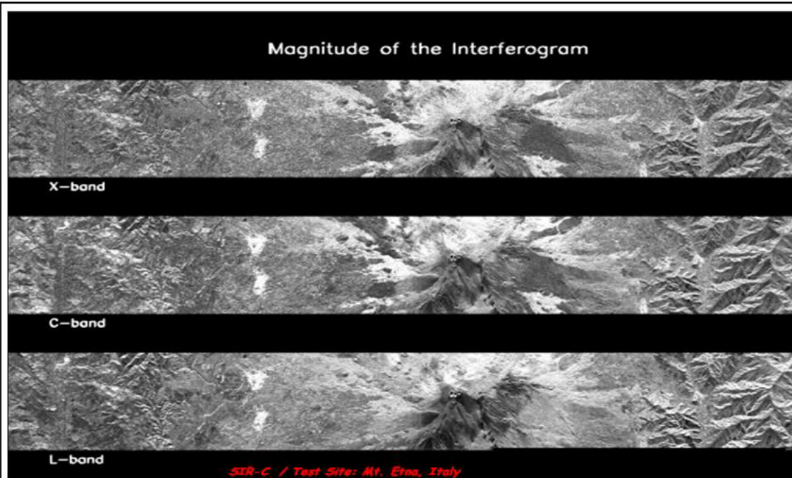
Fig.19 Set of co-registered slant range SAR images in L-, C-, and X-band. The image size is 66.8 km in azimuth and 9 km in ground range (16000 radar pulses and 1024 range bins in X-band and 2048 range bins in L- and C-band).
