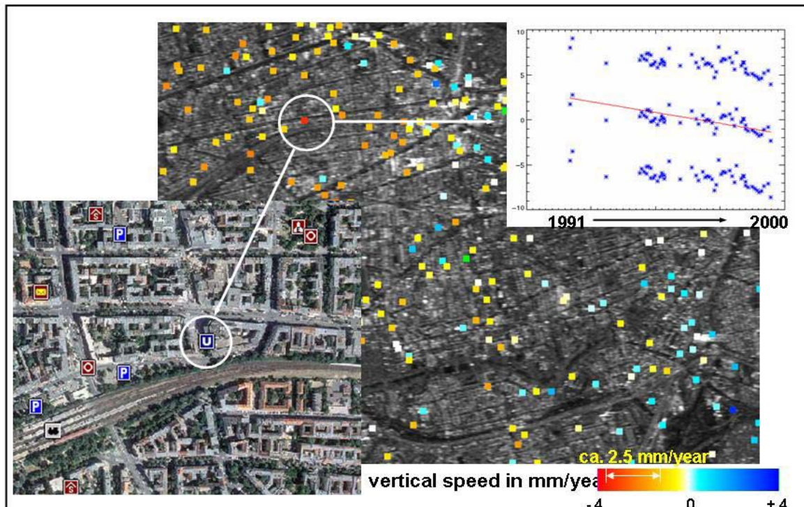
Fig.17 Subsidence rate derived by the PS method. The marked point is a subway station and settles at a velocity of 2.5 mm/year compared to its neighbourhood. 63 ERS data sets from 1991 to 2000 have been used. The plot shows the relatively low noise of the measurement. The \pm 2\sigma ambiguities are plotted for easier interpretation. (Bamler 2000)
