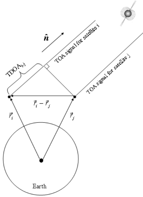
Figure 3.6: TDOA Diagram
