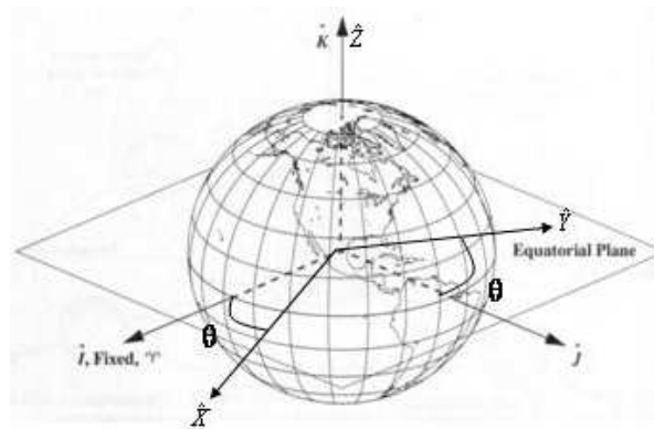
Figure 2.12: The ECEF coordinate system
