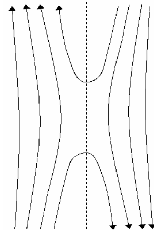
Figure 1.3c – Reconnection and relaxation of magnetic field lines, the dash line in the center represents zero magnetic field where two lines of opposing polarities came into contact and cancelled one another
