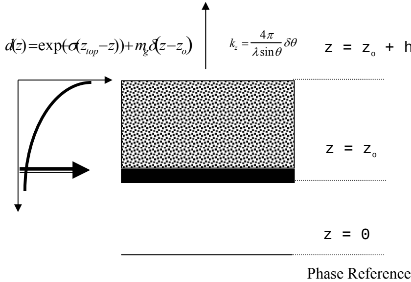
Figure 1: Schematic representation of the 2-Layer coherence model for vegetated land surfaces
