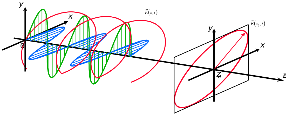
Figure 1a : The Polarisation Ellipse and Spatial helix decomposed into orthogonal components x (horizontal H) and y (vertical V) [Pottier, lectures on polarimetry]
