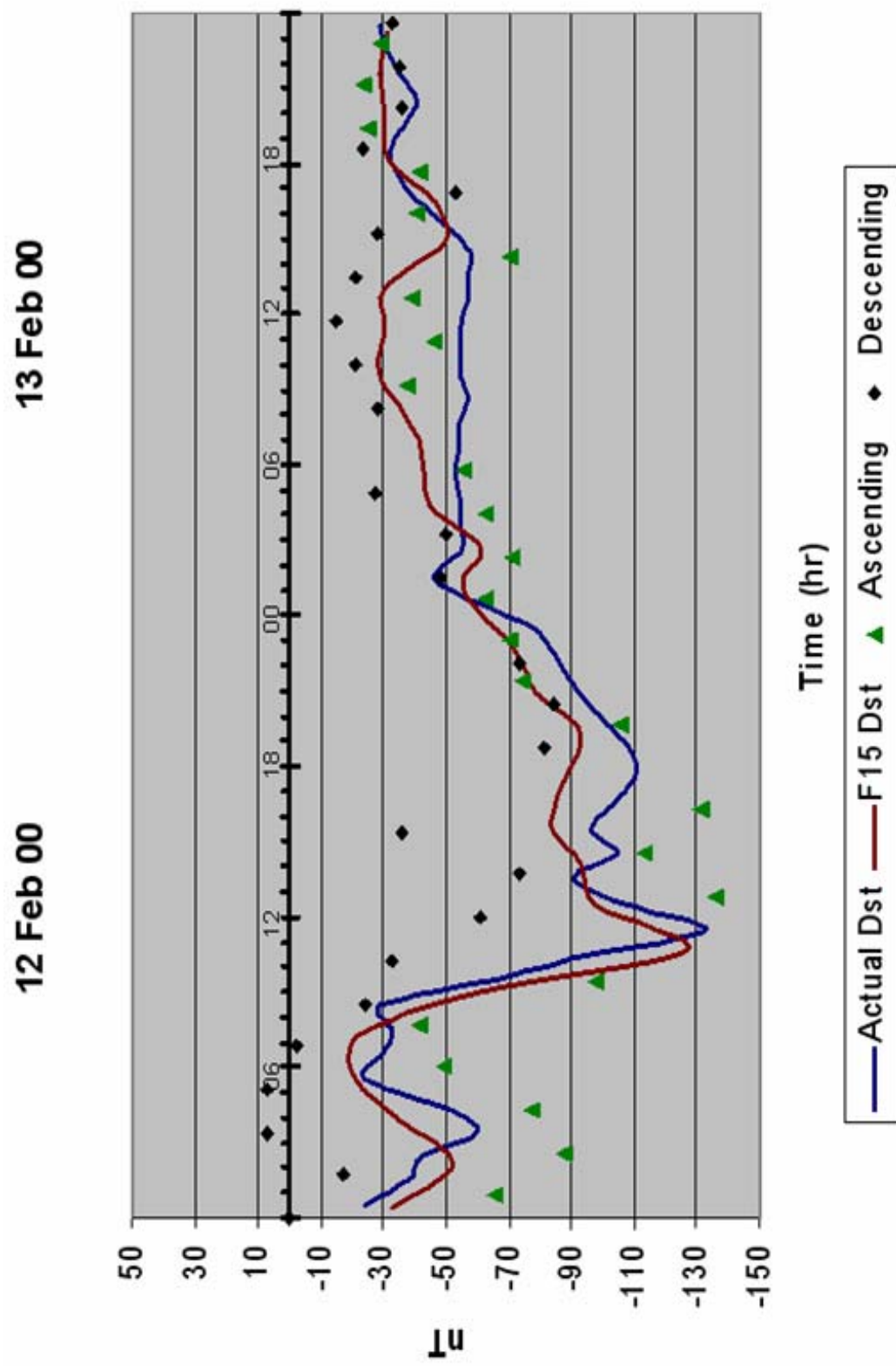
Figure 3.5. Actual vs. DMSP F-15 Dst for 12 -13 February 2000 .
