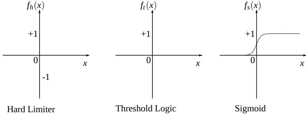
Figure 2: Activation functions
