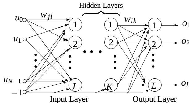
Figure 3: Multi-layer perceptron
