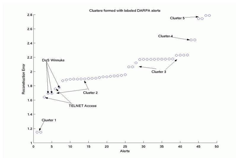
Figure C.1: Reconstruction Error Values
