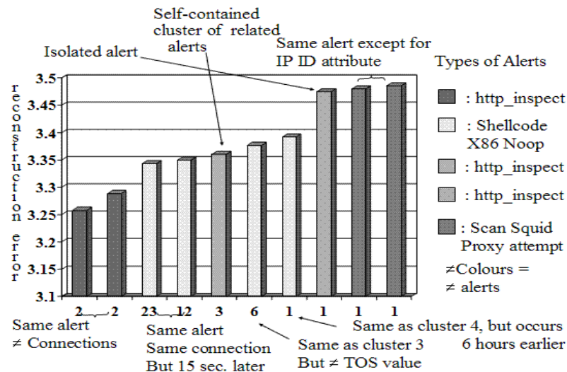
Figure 7: Reconstruction Error Values
