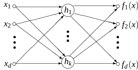
Figure 4: The autoassociator
