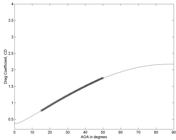
Figure 86: Coefficient of Drag in Free Flow vs Angle of Attack
