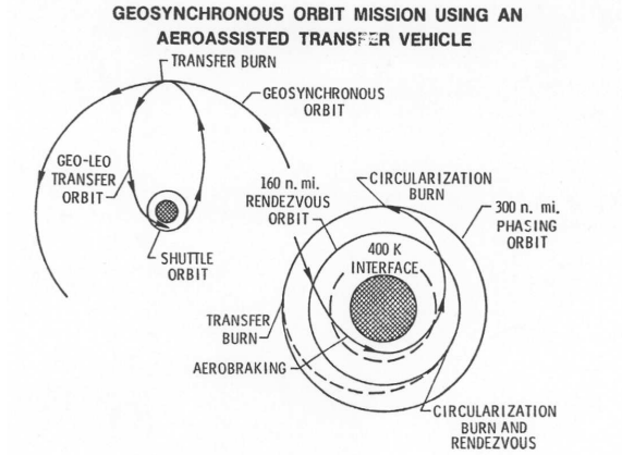
Figure 6: Potential AOTV Aerobreaking Flight Path [15, 46]
