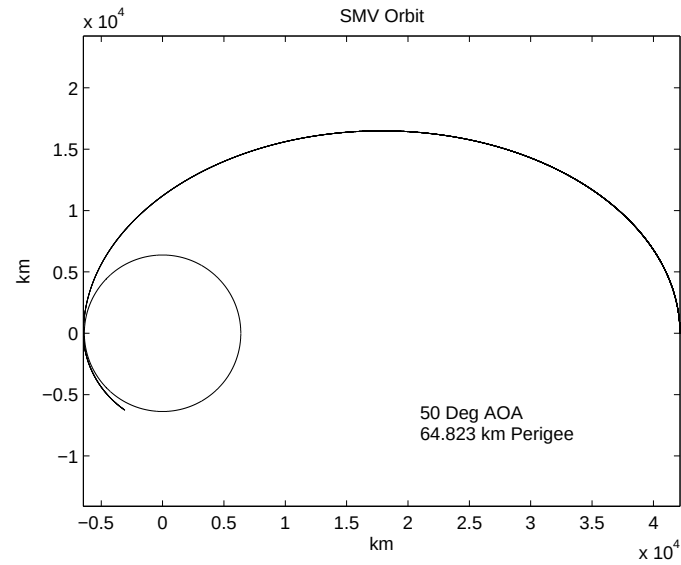
Figure 61: Orbit for 50^\circ AOA, 64.823 km Perigee
