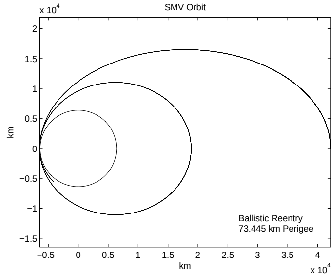
Figure 44: Orbit for Ballistic Reentry, 73.445 km Perigee
