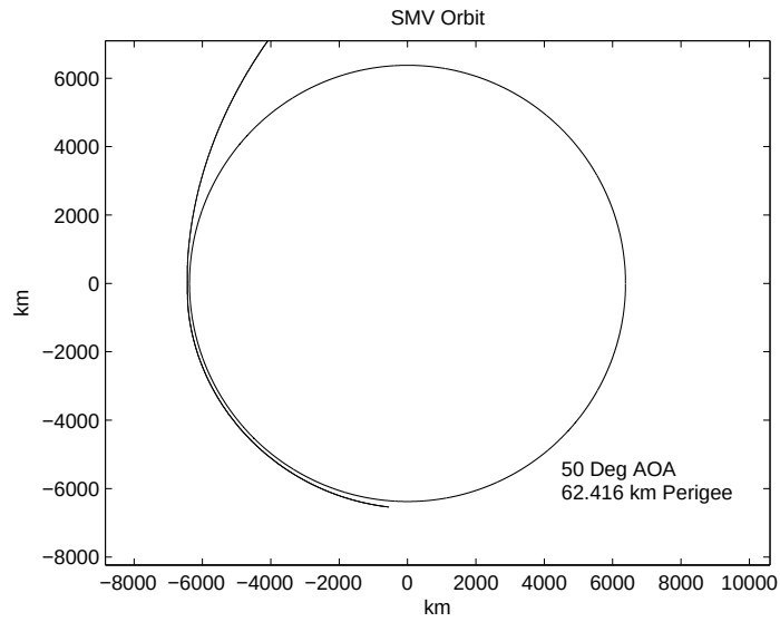
Figure 53: Near Earth Portion of Orbit for 50° AOA, 62.416 km Perigee
