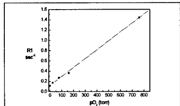
Figure 2 The ^1H spin lattice relaxation rate R_1 of HMDSO varies linearly with oxygen tension ( pO_2 ). At 40 ^{\circ}C , R_1 = 0.12 + 0.00173 \cdot pO_2 (torr)
