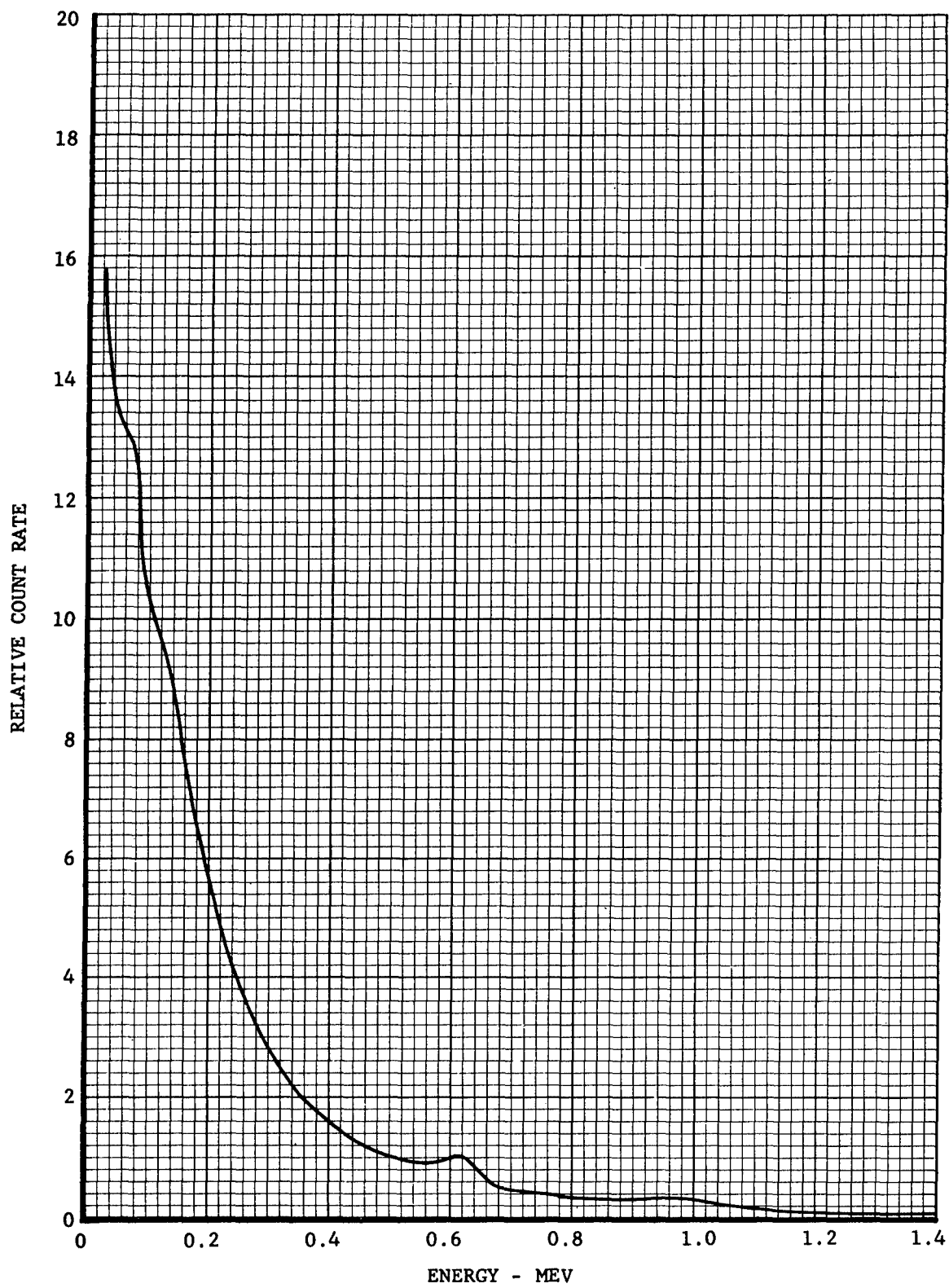
Fig. 3.5—Pulse-height distribution at position B from 16.3-curie \text{Co}^{60} source.
