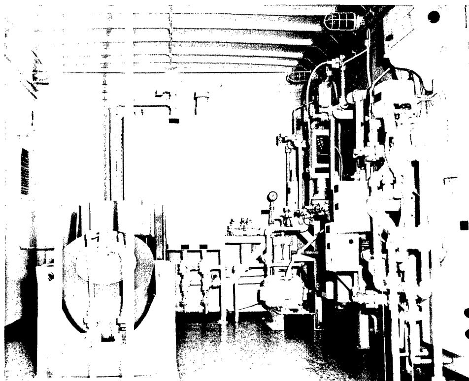
Fig. 2.4—Interior of source truck showing shields and pumping system.
