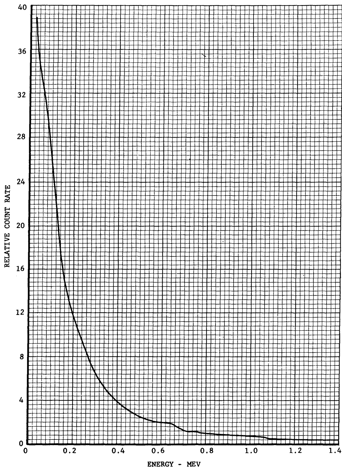
Fig. 3.3—Pulse-height distribution at position A from 196-curie \text{Co}^{60} source.
