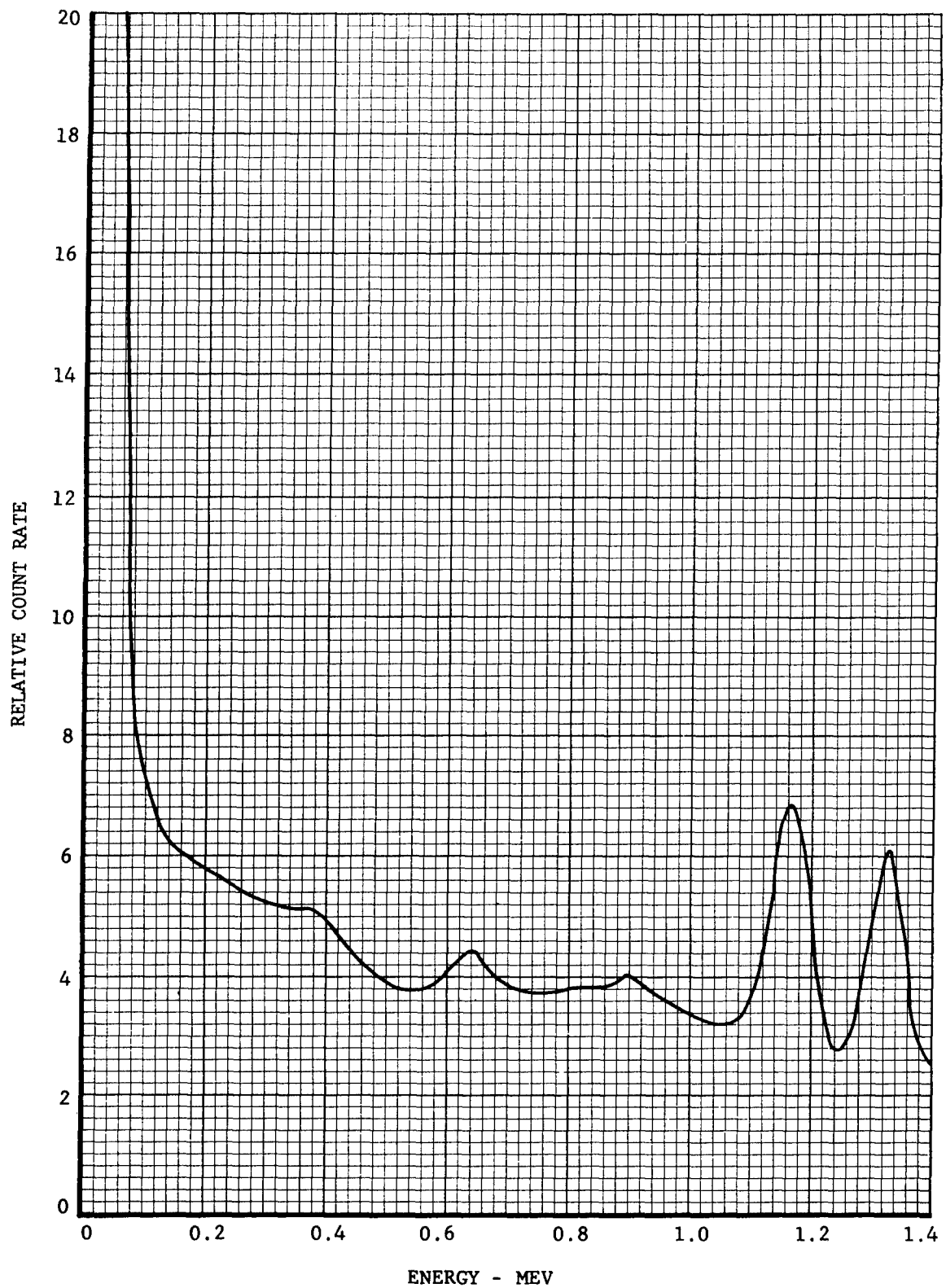
Fig. 3.1—Pulse-height distribution from \text{Co}^{60} standard.
