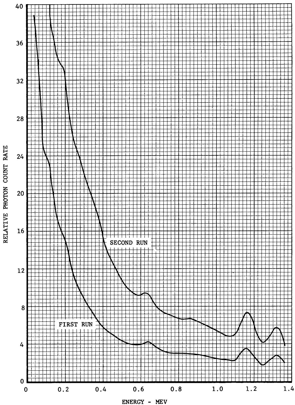
Fig. 3.2—Pulse-height distribution 3 ft above rectangular area source.
