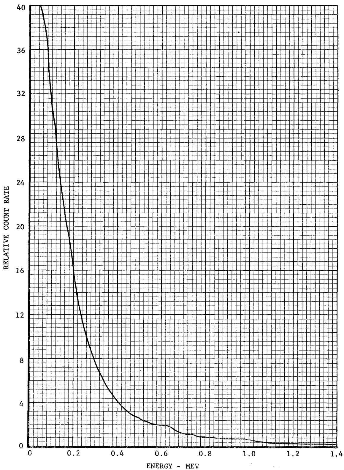
Fig. 3.3—Pulse-height distribution at position C from 16.3-curie \text{Co}^{60} source.
