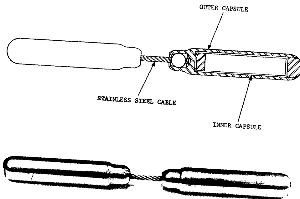
Fig. 2.8—The 200-curie \text{Co}^{60} source capsule.
