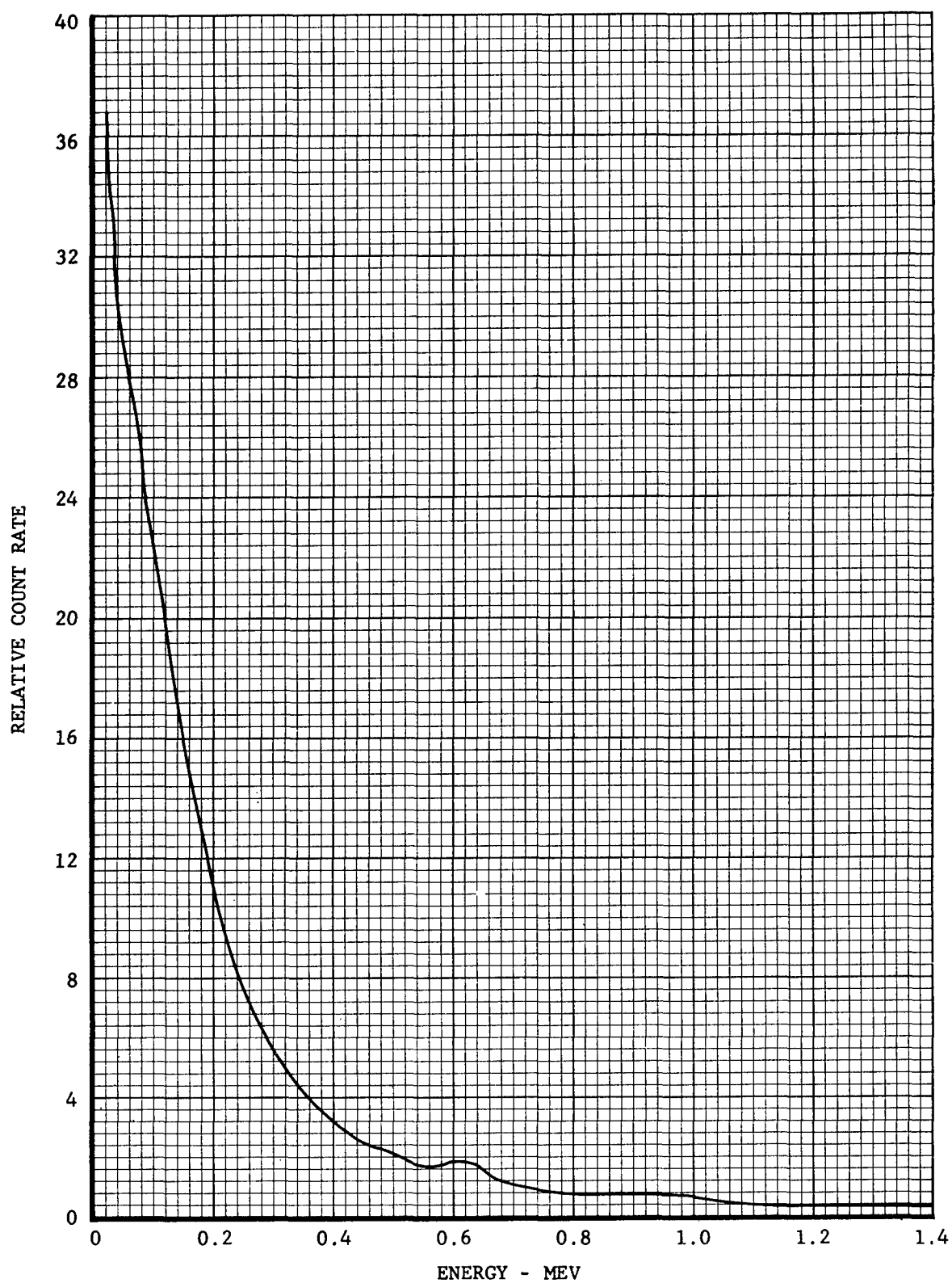
Fig. 3.4—Pulse-height distribution at position B from 196-curie \text{Co}^{60} source.
