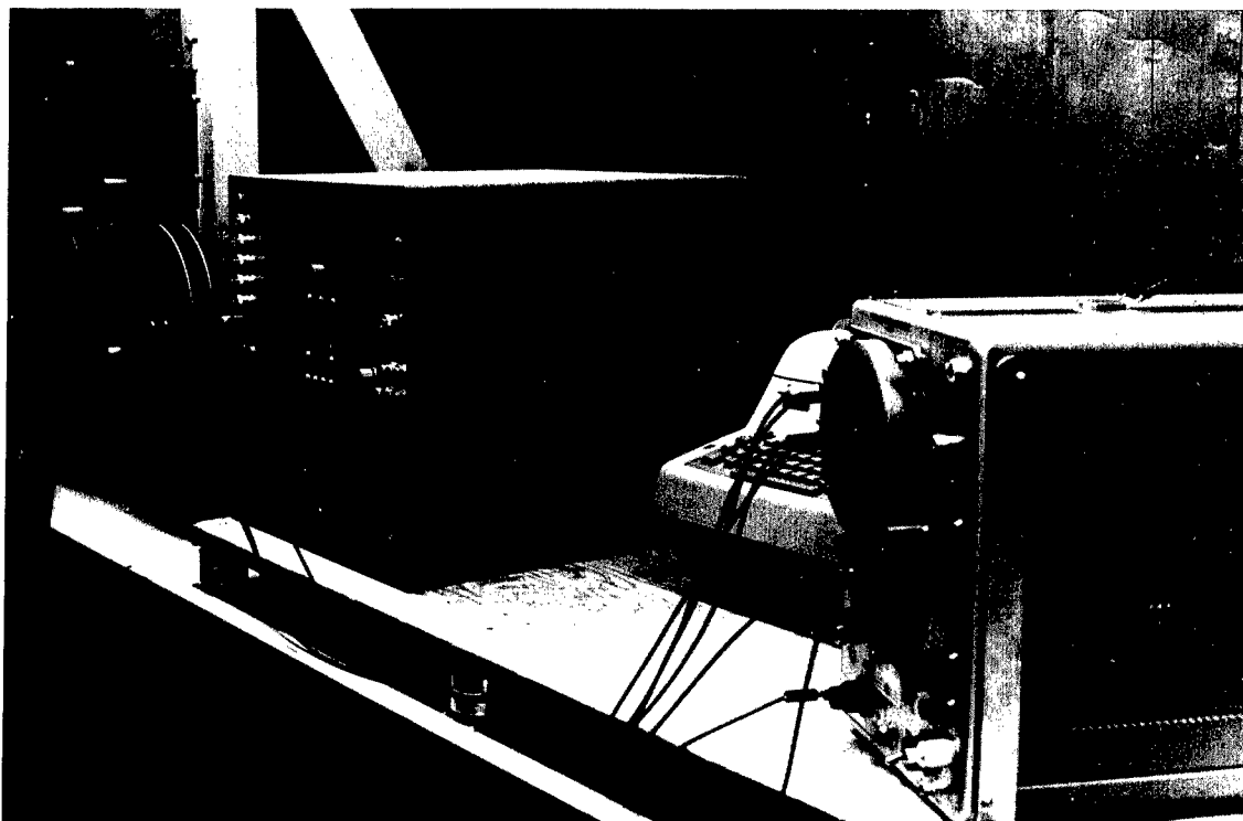
Fig. 3.9—Shock-mounted instruments, interior of shielded mobile laboratory.
