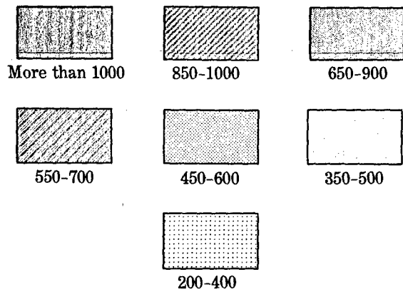
Generalized levels of aeroradioactivity, in counts per second
