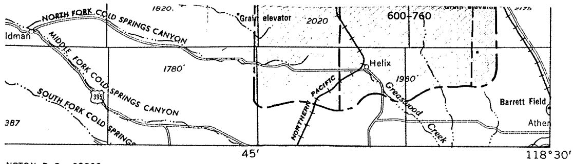
Aeroradioactivity survey made at 500 feet above the ground under the direction of J. L. Meuschke and P. W. Philbin, 1959
