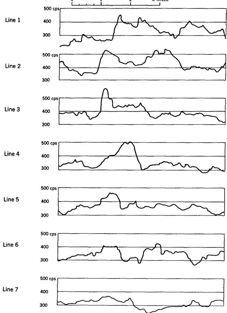
AERORADIOACTIVITY PROFILES ALONG LINES 1-7, LOOKING WEST
