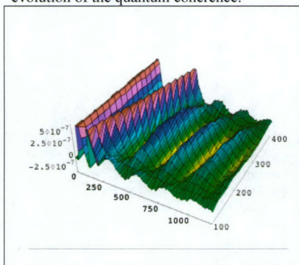
Figure 13. Experimental results demonstrating coherent optical control of electron spin coherence. The x-axis represent the time evolution of the quantum coherence showing quantum beats similar to Fig. 8. The y-axis represent the phase delay (in time) between the spin coherence forming pulse and the control pulse. Constructive interference is seen around a phase delay of 300.
