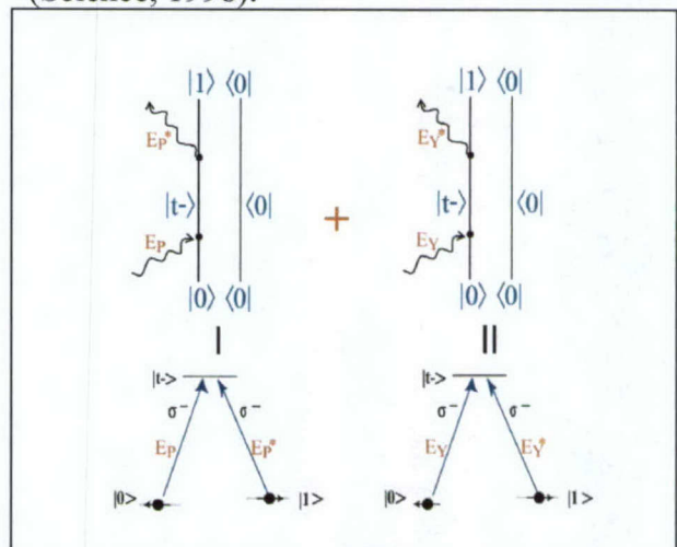
Figure 12. Double side Feynman diagrams showing the origin of coherent optical control of spin. This control is achieved by the interference of two optically excited pathways leading to production of spin coherence between the two spin states.
