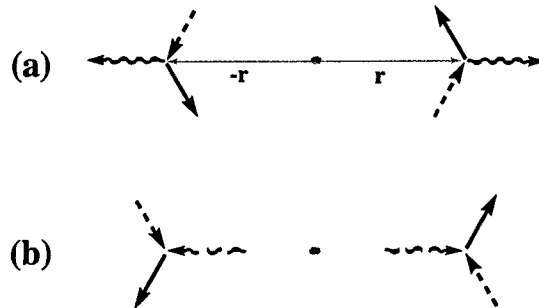
Figure 3: Examples of long-range collisions that locally conserve mass, momentum, and energy. |\Delta p| = \pm 1 interactions along the r_0 -direction coupled to a heat bath: (a) attractive case; and (b) its adjoint, repulsive case. Transition probabilities for these collisions have a Monte Carlo form as they are biased by the density of heat-bath particles, rendered here with wavy lines. Head of the gray arrows indicates particles entering the sites at r_0 and -r_0 at time t . Tail of the black arrows indicates particles leaving those sites at time t + \tau .
