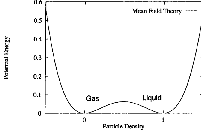
Figure 2: Potential energy versus particle density in the zero temperature limit. Letting d \rightarrow \psi - \frac{1}{2} , then V(\psi) = \frac{1}{16} - \frac{1}{2}\psi^2 + \psi^4 which has a Landau-Ginsburg form.
