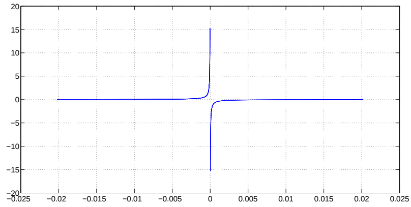
Figure 3: Two branches of \alpha \hat{z} = \pm \sqrt{r} \exp i \frac{\theta}{2} . Vertical axis denotes real part of \alpha \hat{z} , horizontal axis denotes imaginary part of \alpha \hat{z} .
