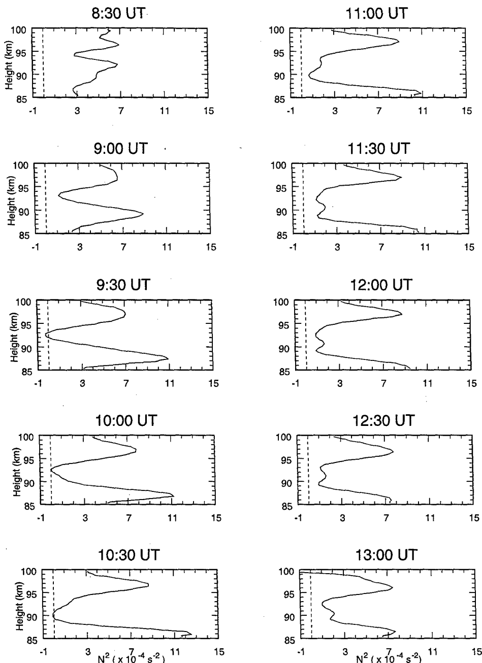
Figure 1. The vertical profile of Brunt-Väisälä frequency squared, N^2 , from 0830 to 1030 UT are plotted in the first column and 1100 to 1300 UT in the second column. The dashed vertical line indicates where N^2 becomes zero.
