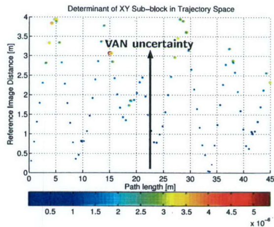
(d) VAN uncertainty represented as a scatter plot.
