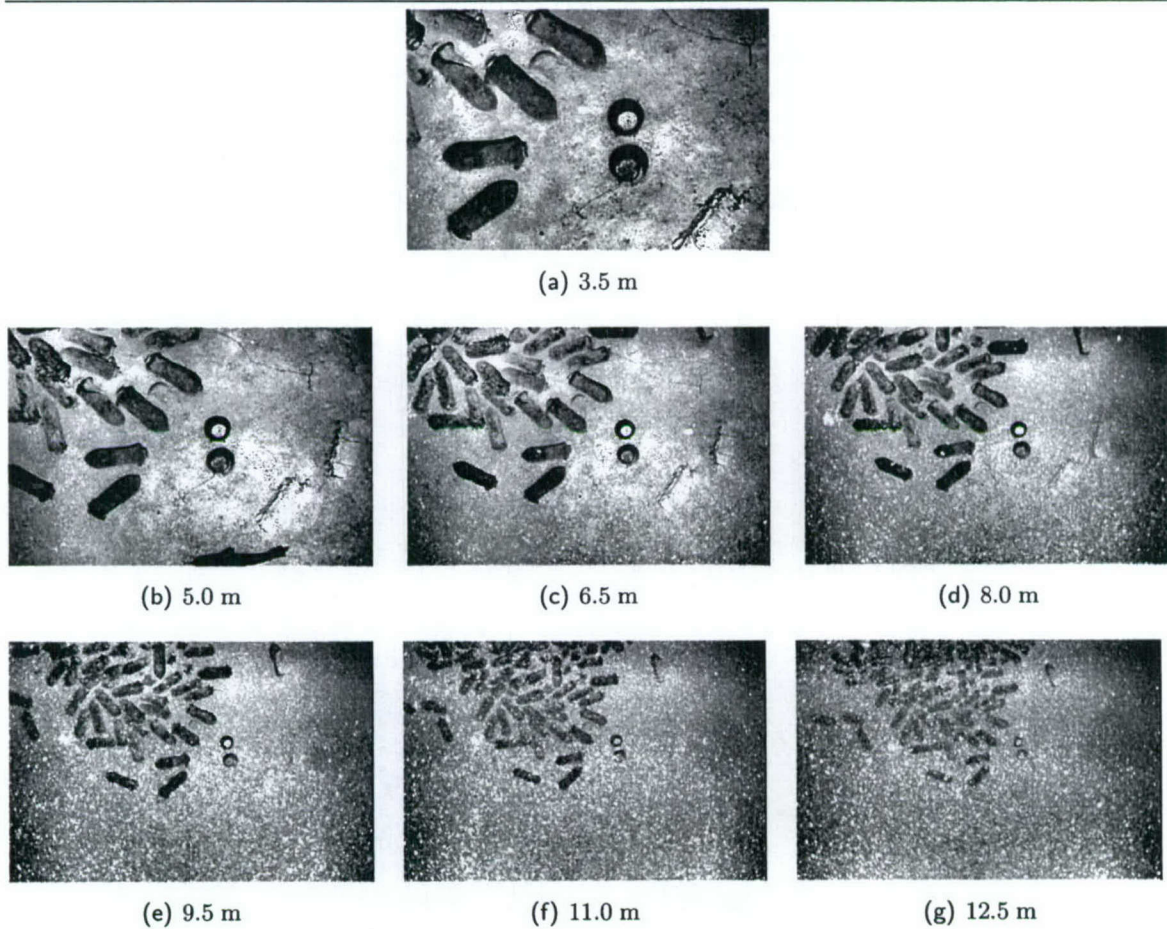
Figure 1-12 A demonstration of underwater backscatter using data collected by the Jason ROV [149]. In this example, a sequence of images is shown over an incremental range of altitudes to demonstrate the significance of backscatter in the underwater imaging process. Note that backscatter reduces the effective altitude at which an underwater vehicle can clearly image the scene. Practical camera-to-light separations for a typical AUV platform dictate that it must fly within several meters of the seafloor in order to find a tolerable tradeoff between backscatter and imaged FOV.
