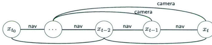
(b) Conceptual illustration of the measurement constraints (Markov network).
