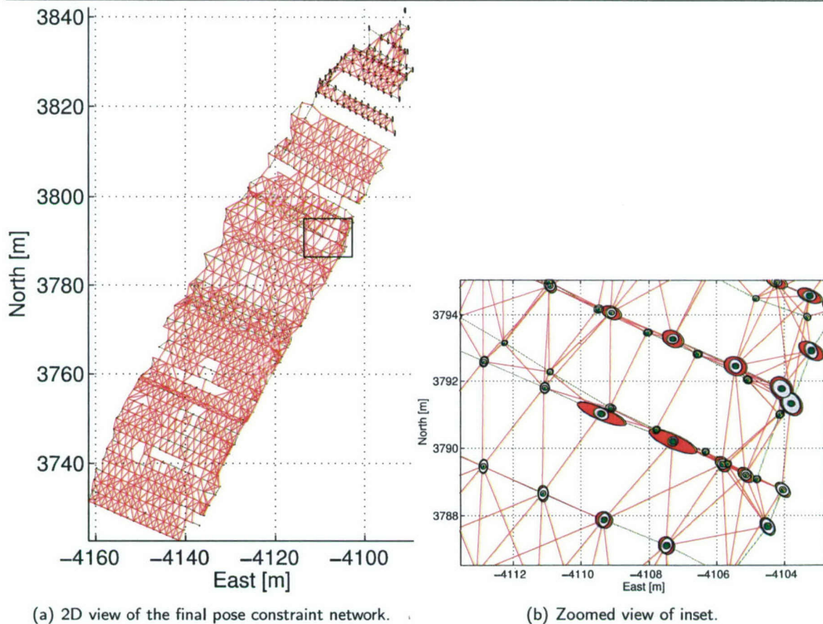
Figure 4-10 The recovered XY trajectory and covariance bounds for the RMS Titanic. (a) Final XY pose constraint-network associated with using 866 images to provide 3494 camera constraints; 3-sigma bounds are shown. (b) A zoomed view illustrating the consistency of the data association bounds generated by our algorithm. Note that for this plot the 3-sigma bounds have been inflated by a factor of 30 for visualization. In this plot we have: 1) the initial covariance bounds associated with pose insertion (red), 2) the marginal covariance bounds based upon constant-time Kalman updates (gray), and 3) the actual marginal covariance bounds obtained by matrix inversion (green). Note that all of the estimated bounds (gray) were verified to be consistent with respect to the actual marginal covariance (green) by performing Cholesky decomposition on their difference to establish positive definiteness. The reason why some of the estimated covariance bounds (gray) are tighter approximations than others to the actual filter bounds (green) is because our algorithm only updates the bounds on a per re-observation basis. Hence, if the robot is sufficiently well-localized when it re-observes an image, then the covariance bound of the corresponding delayed-state improves.
