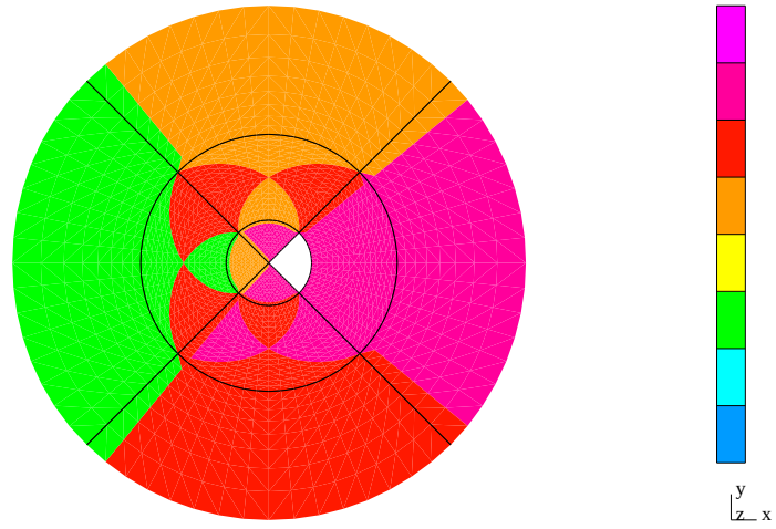
Figure 12: Scattering of a plane wave on a wedge. Optimal hp mesh for the direction of 90 degrees
