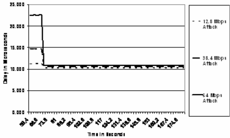
Figure 25 – Router Queuing Delay of 40 Mbps Pipe
