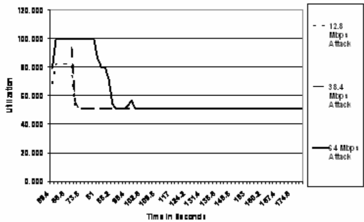
Figure 30 – Inbound Bandwidth Utilization of 40 Mbps Pipe
