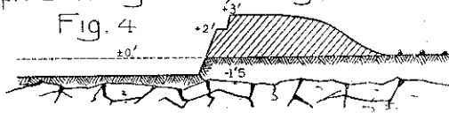
Simple Standing Trench, Rocky Ground
