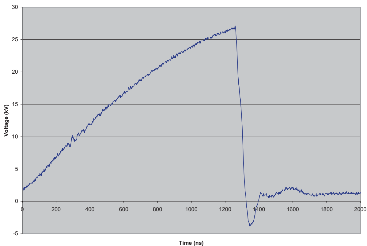
Fig. 5 — Explosively generated voltage pulse
