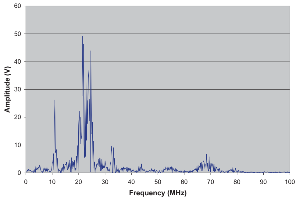
Fig. 8 — FFT of the received signal
