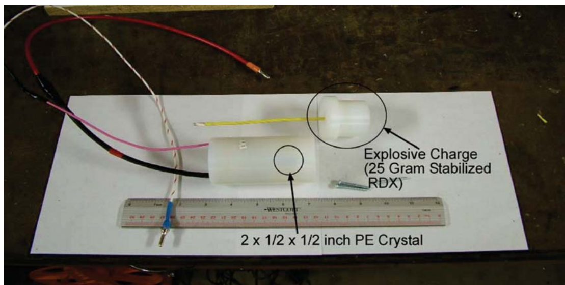
Fig. 1 — Loki FEG ready for assembly
