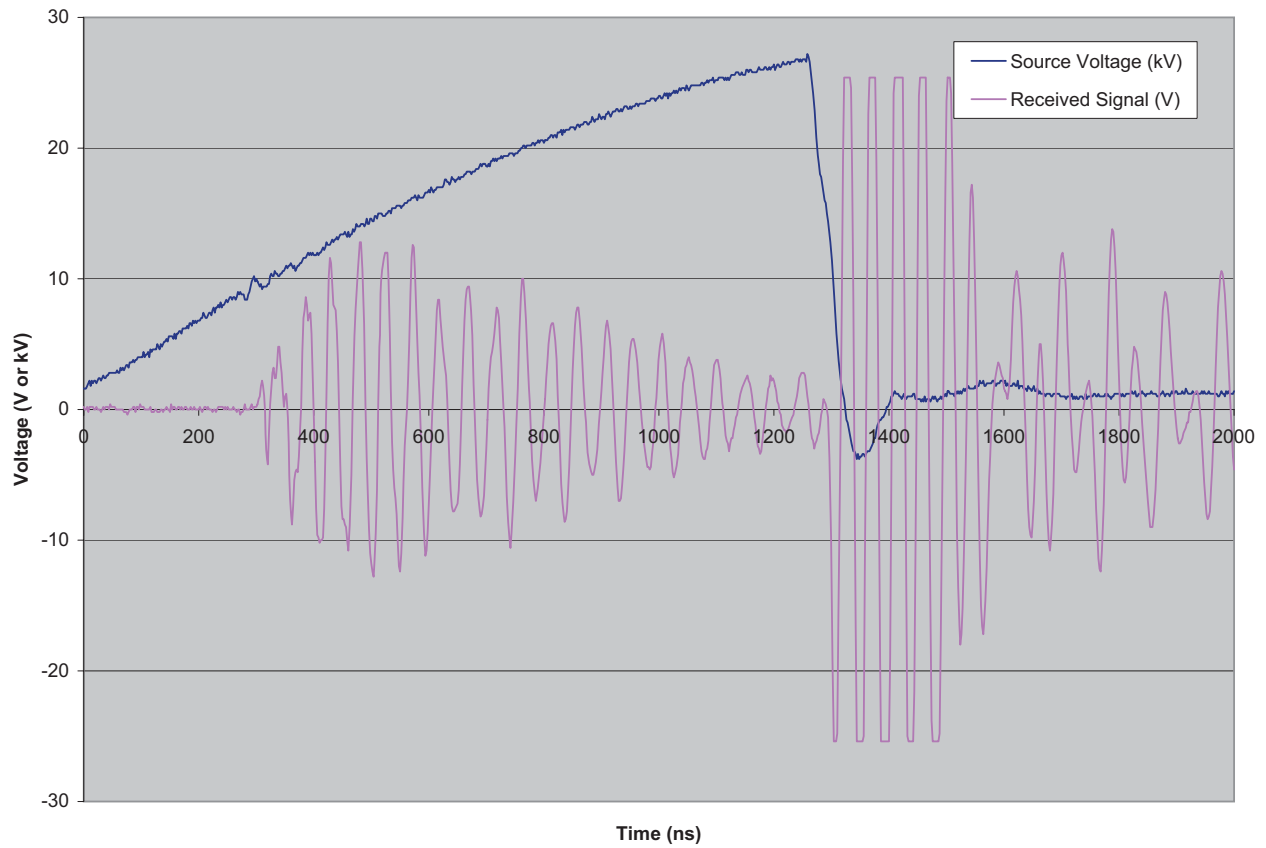
Fig. 7 — Receiver antenna signal and source voltage
