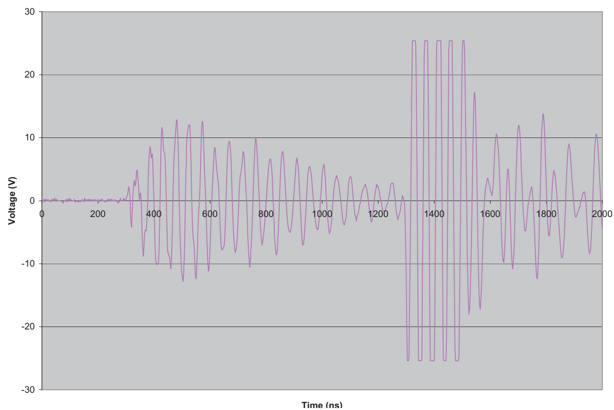
Fig. 6 — Explosively driven RF signal received 3 m from the transmitting antenna
