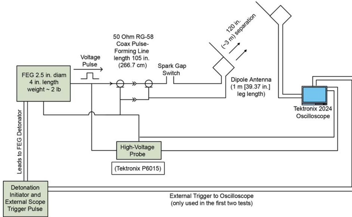
Fig. 4 — RF generation and measurement layout
