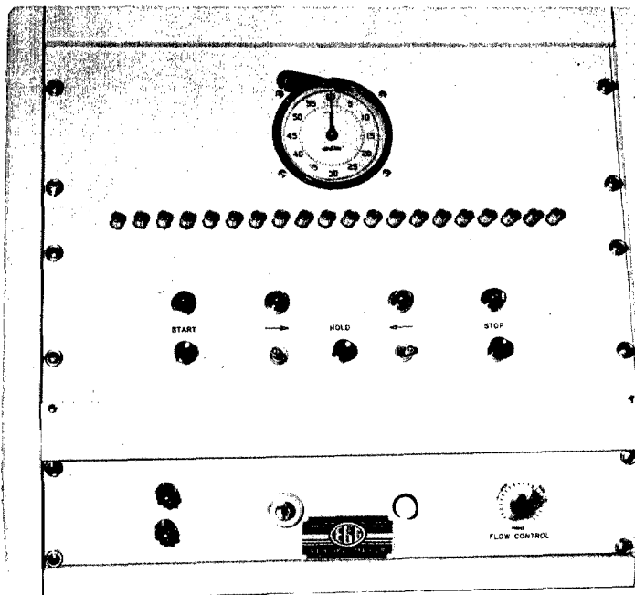
Fig. A.6—Remote-control console.
