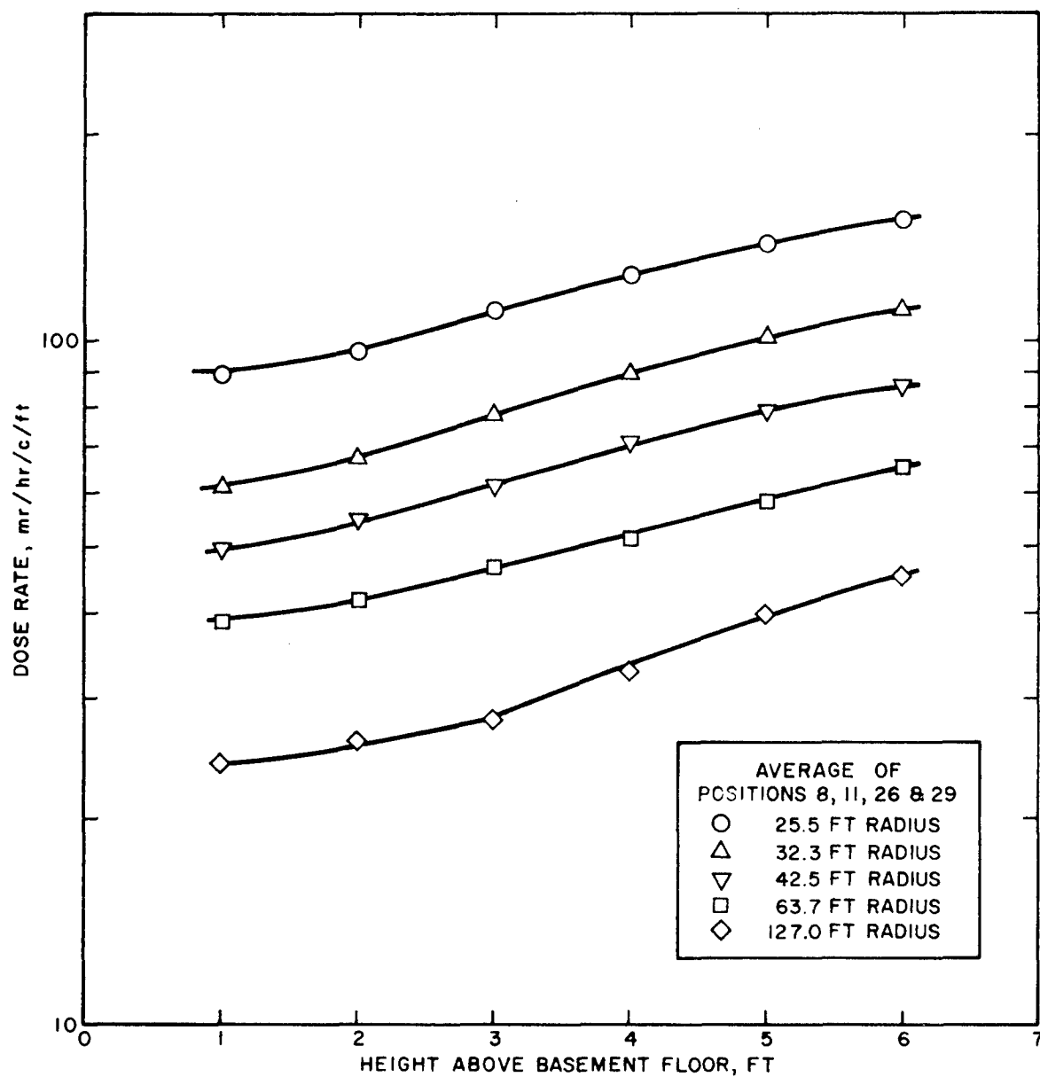
Fig. 3.5—Normalized dose rate from ring sources in Butler building (positions 8, 11, 26, and 29).
