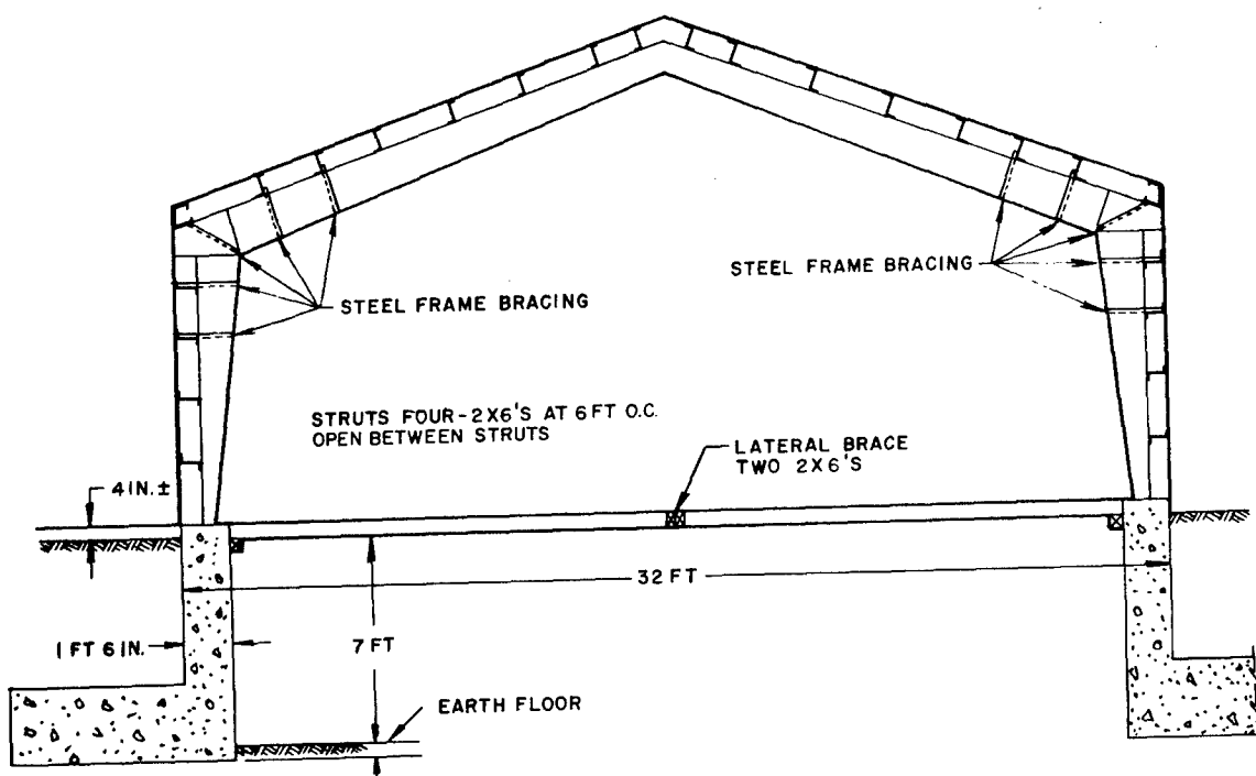
Fig. 1.2 — Typical transverse section of Butler building.
