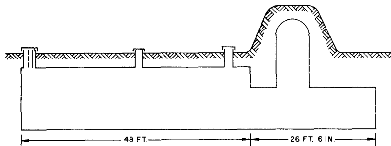
SIDE VIEW SHOWING ENTRANCE
