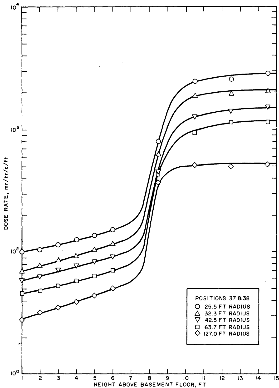
Fig. 3.3—Normalized dose rate from ring sources in center of Butler building (positions 37 and 38).
