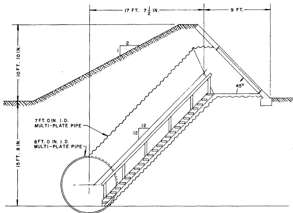
Fig. 1.5—Stairway to entrance of underground group shelter.
