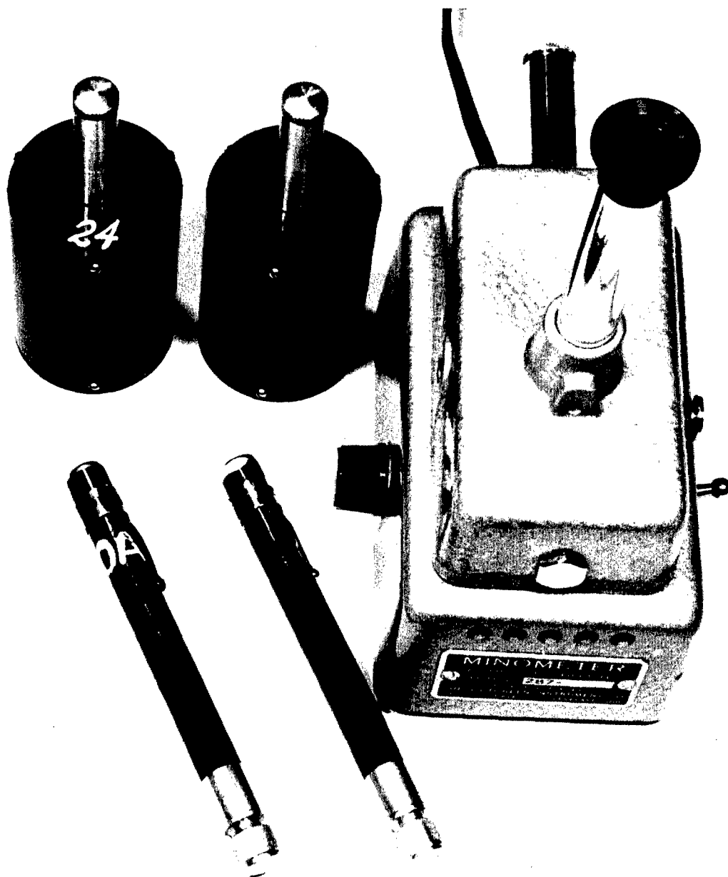
Fig. A.9— Ionization chambers and charger-reader.
