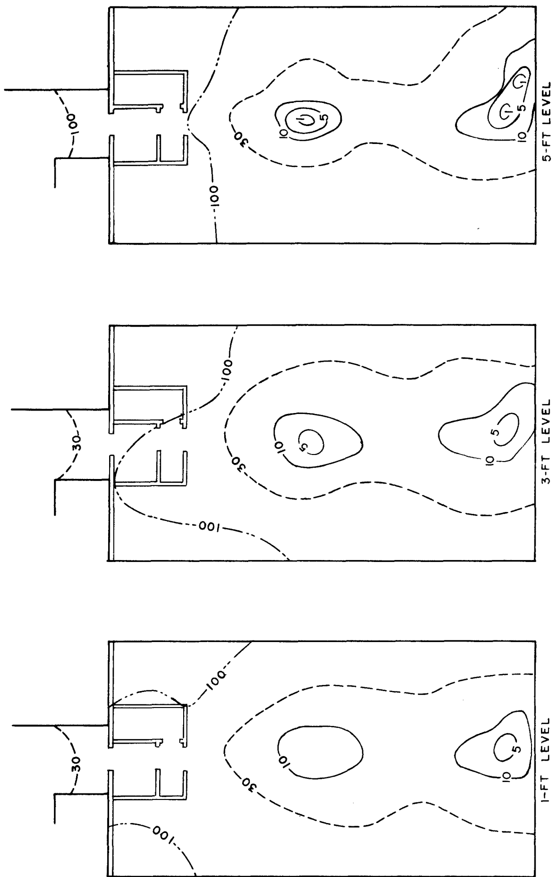
Fig. 4.5—Protection factors at three heights in underground group shelter (multiply by 1000).
