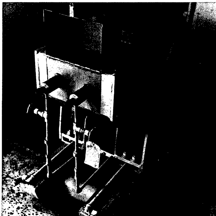
Fig. A.3—Large \text{Co}^{60} source shield.
