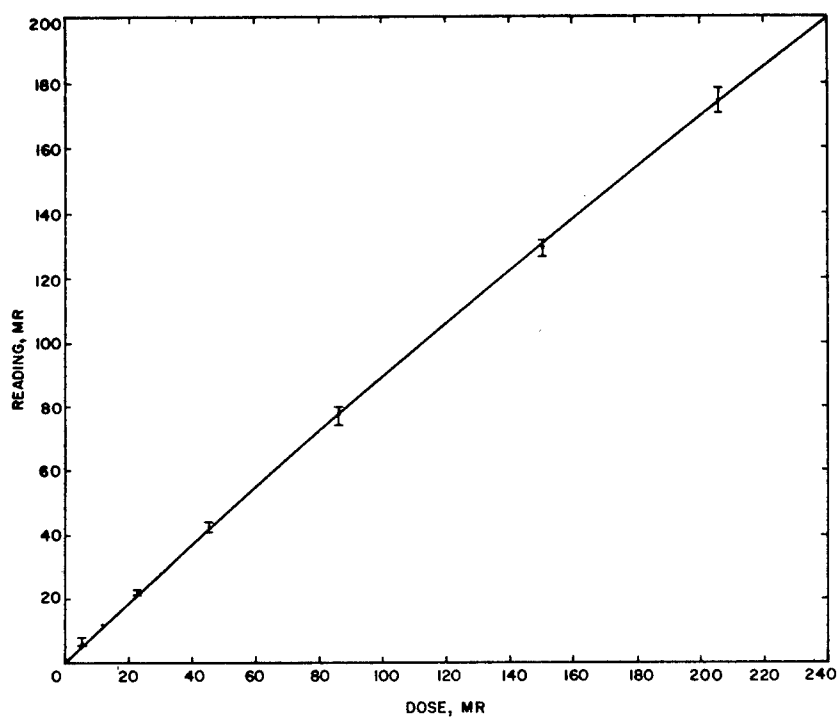
Fig. A.10—Calibration curve for the Victoreen model 362 ionization chamber.
