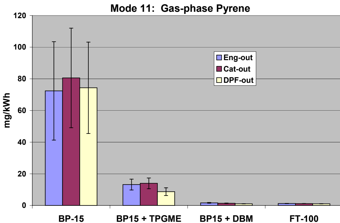
Figure C-17. Gas-Phase Pyrene Emissions by Fuel Type, Mode 11
