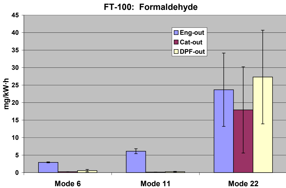
Figure H-16. Formaldehyde Emissions with Fischer-Tropsch Fuel
