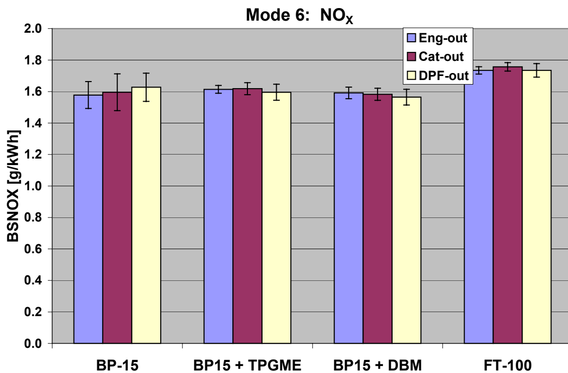
Figure B-10. Nitrogen Oxides Emissions by Fuel Type, Mode 6
