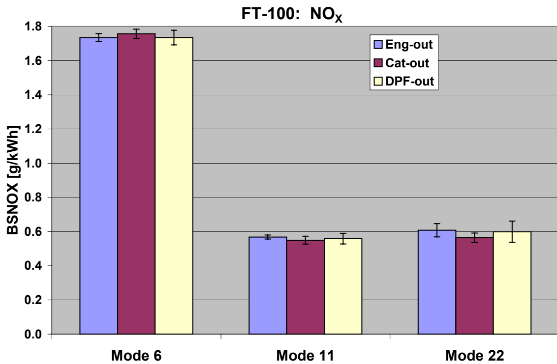
Figure H-10. Nitrogen Oxides Emissions with Fischer-Tropsch Fuel
