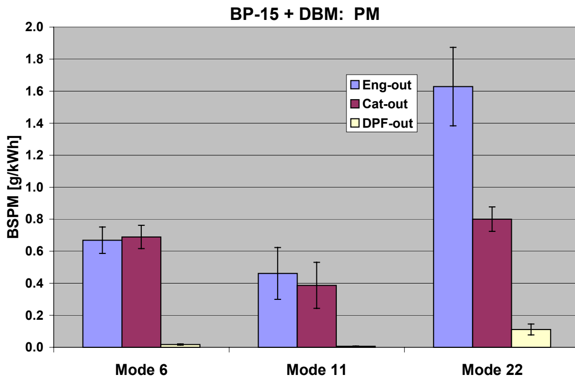
Figure F-11. Particulate Matter Emissions with DBM Fuel Additive
