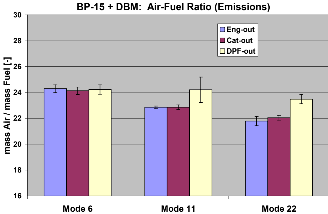
Figure F-3. Emissions Air-Fuel Ratio with DBM Fuel Additive
