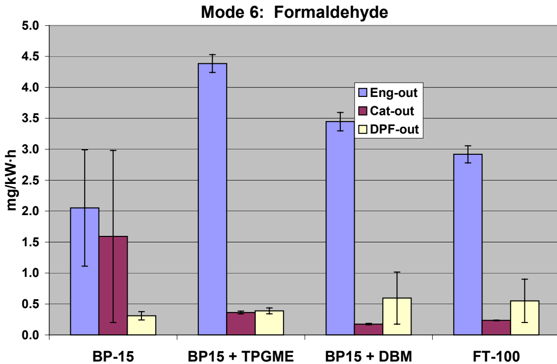
Figure B-16. Formaldehyde Emissions by Fuel Type, Mode 6
