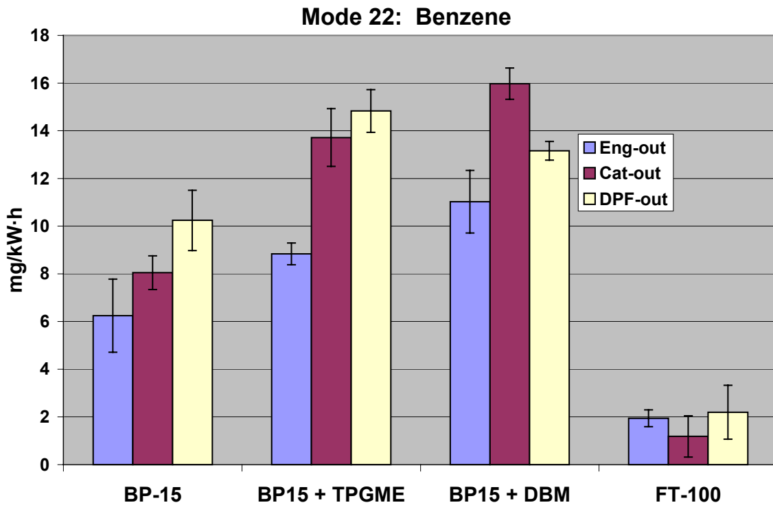
Figure D-14. Benzene Emissions by Fuel Type, Mode 22
