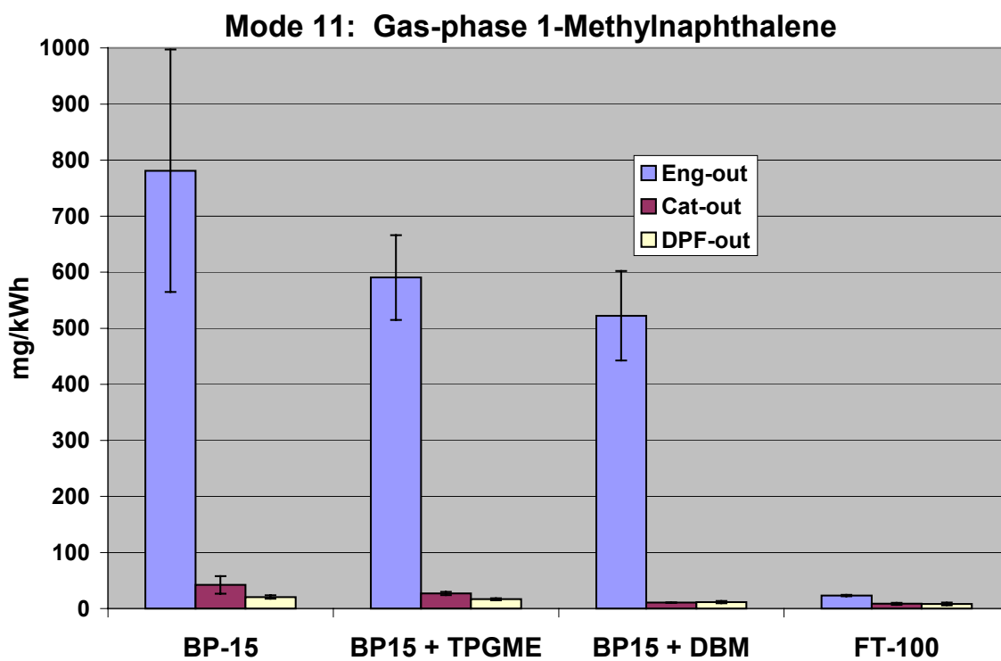
Figure C-26. Gas-Phase 1-Methylnaphthalene Emissions by Fuel Type, Mode 11
