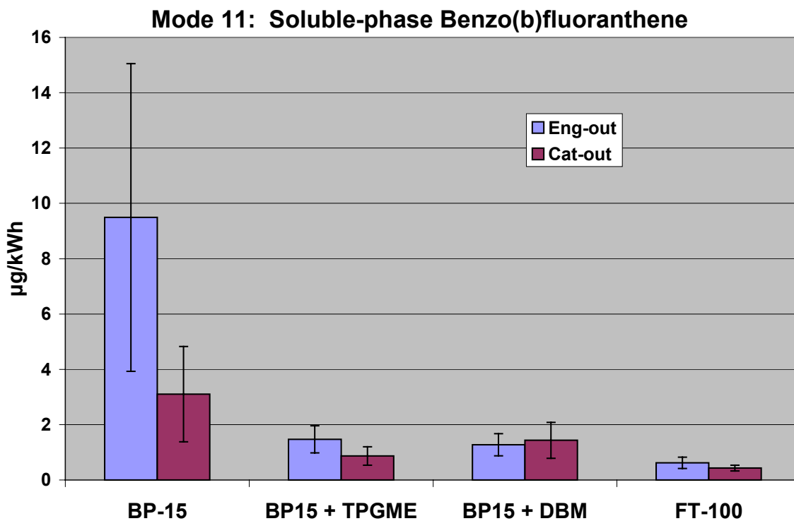
Figure C-35. Soluble-Phase Benzo(b)fluoranthene Emissions by Fuel Type, Mode 11
