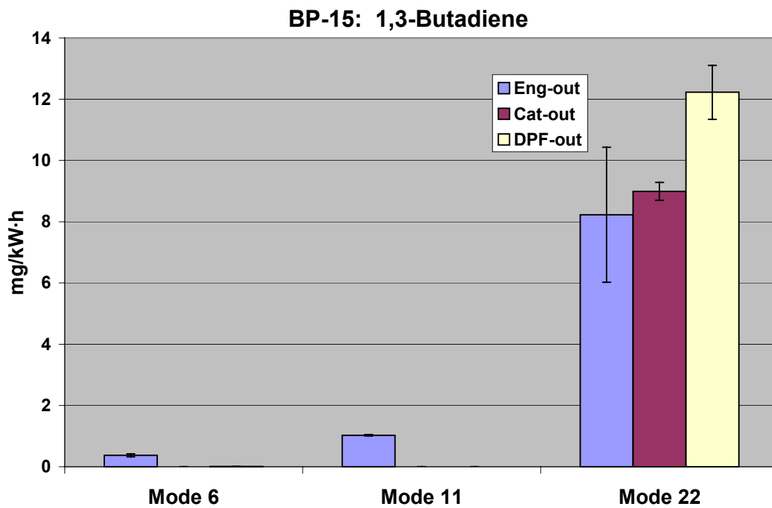
Figure E-13. 1,3-Butadiene Emissions with BP-15 Fuel
