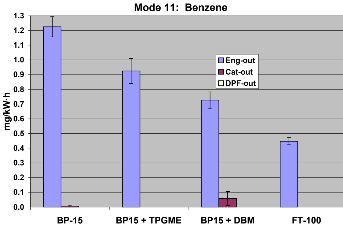
Figure C-14. Benzene Emissions by Fuel Type, Mode 11
