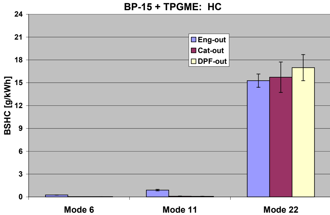
Figure G-9. Hydrocarbon Emissions with TPGME Fuel Additive
