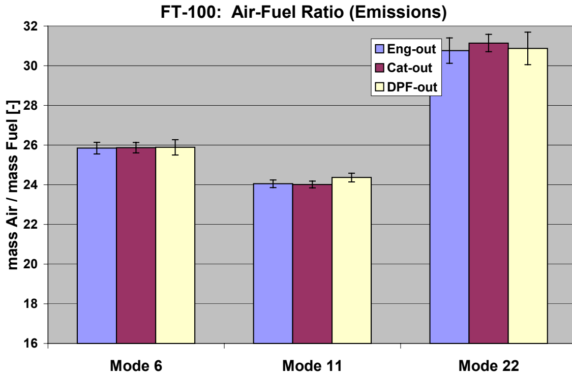
Figure H-3. Emissions Air-Fuel Ratio with Fischer-Tropsch Fuel
