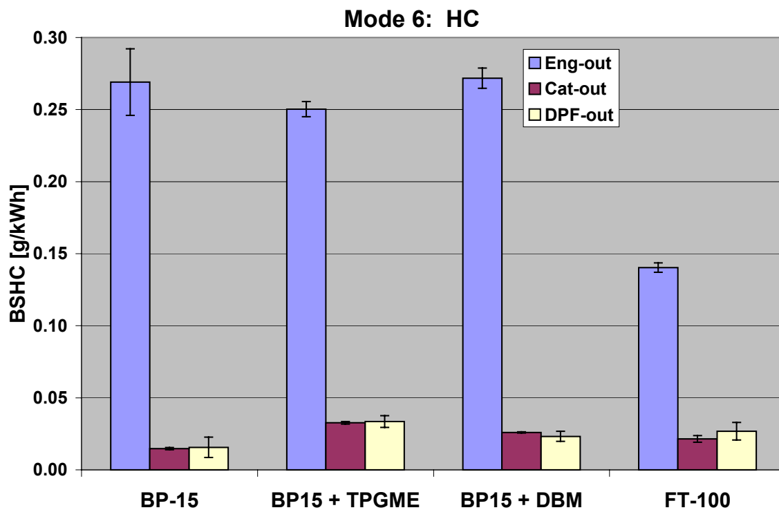
Figure B-9. Hydrocarbon Emissions by Fuel Type, Mode 6
