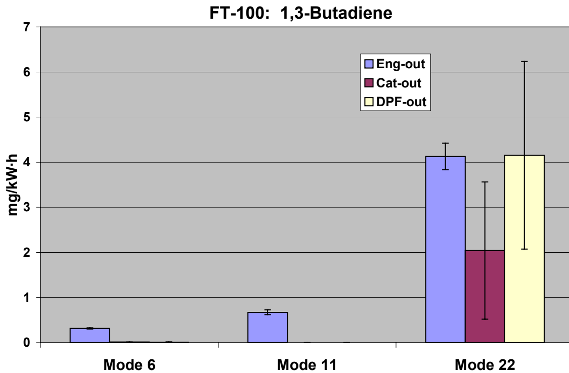
Figure H-13. 1,3-Butadiene Emissions with Fischer-Tropsch Fuel
