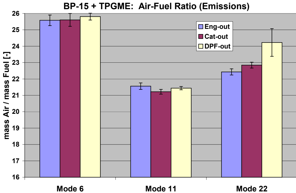
Figure G-3. Emissions Air-Fuel Ratio with TPGME Fuel Additive
