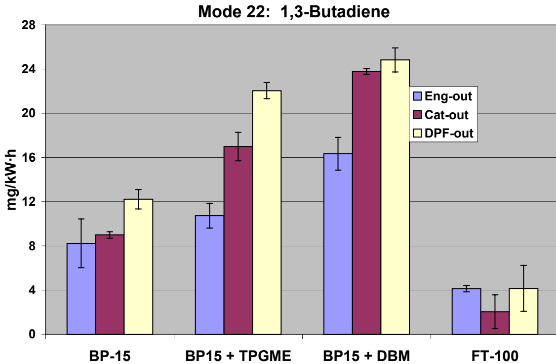
Figure D-13. 1,3-Butadiene Emissions by Fuel Type, Mode 22
