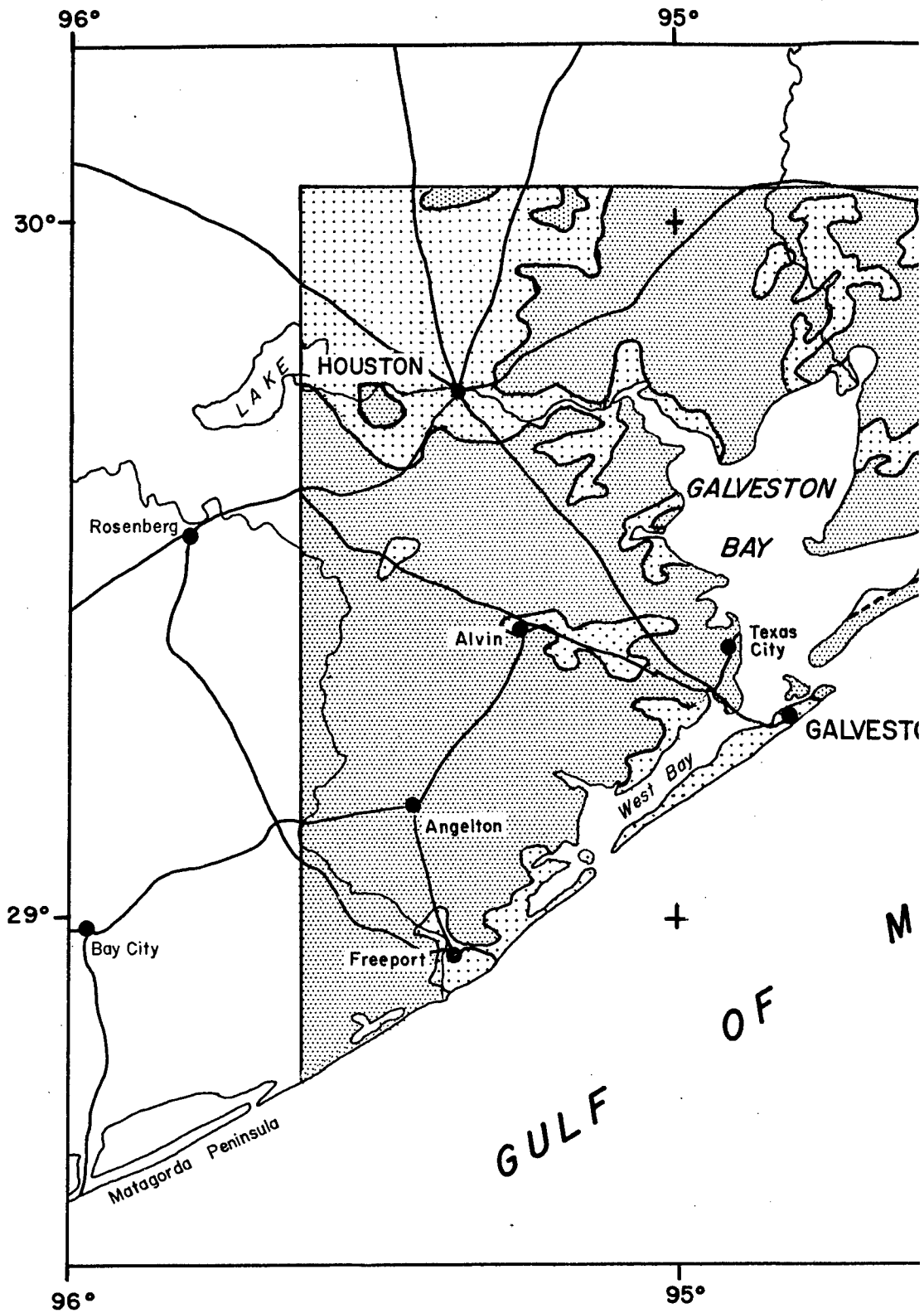
Fig. 5—Generalized aeroradioactivity map of the ARMS-II Galveston, Tex., area. Radioactivity by Edgerton, Germeshausen & Grier, Inc., Jan. 27 to Feb. 17, 1962, with aircraft N702B.)
