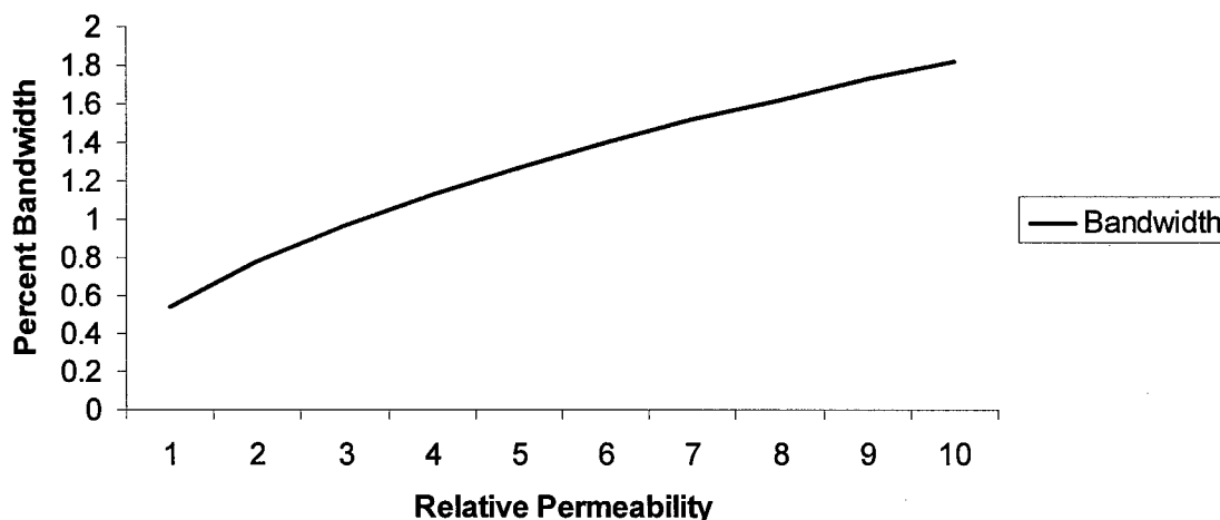
Figure 3. Patch antenna bandwidth for a relative permittivity of five vs. relative permeability. Bandwidth is one of the key parameters that determine the utility of an antenna. Air Force applications now routinely use wide bandwidth apertures. In the example above, the bandwidth of the antenna nearly quadrupled compared to the non-magnetic case. Further examples are given in [7]. Note that the material provided (heavily-loaded NiFe composite in a urethane matrix that used large inclusions – ~45 microns) was definitely not low loss and hence the realized bandwidth was due more to loss than permeability.
