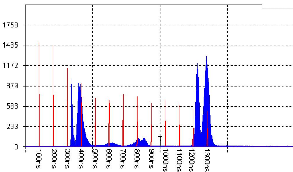
Figure 74: TAC output with PSA A-channel constant fraction setting of 10%
