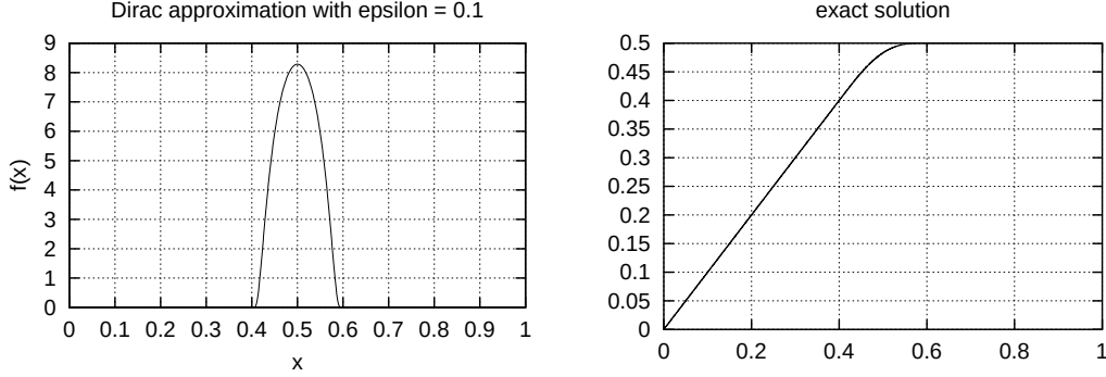
Figure 7: Representation of the load (left) and the exact solution (right).
