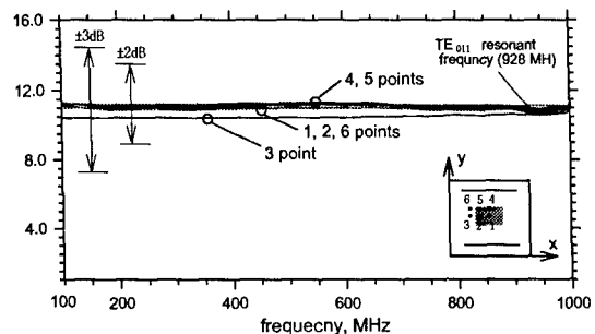
Fig.2. Measured electric fields inside the designed SCTL cell ( P_1 = 7\text{dBm} )
