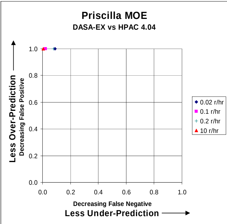
Figure 27. MOE - Priscilla, DASA-EX vs. HPAC 4.04
