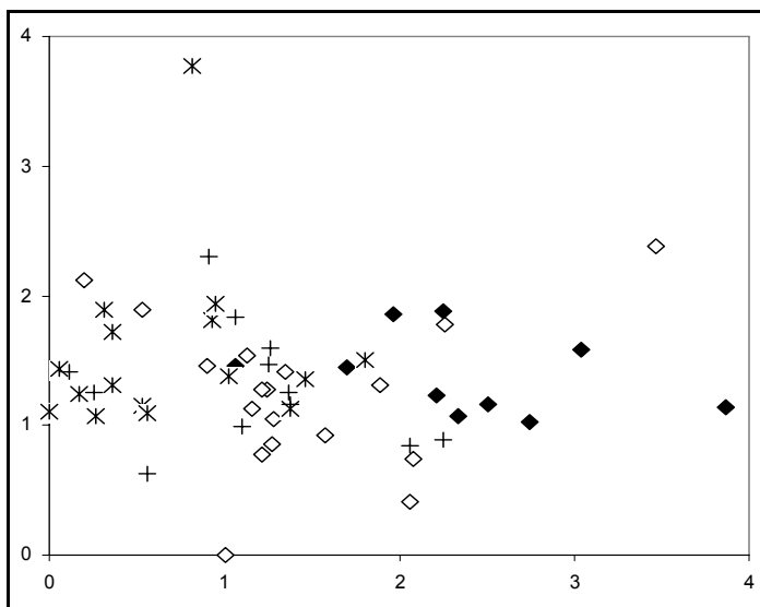
Figure 5. Detrended correspondence analysis (DCA) site biplot of intermittent and perennial springs and headwater sites in the River Lathkill catchment (1998-2000)
