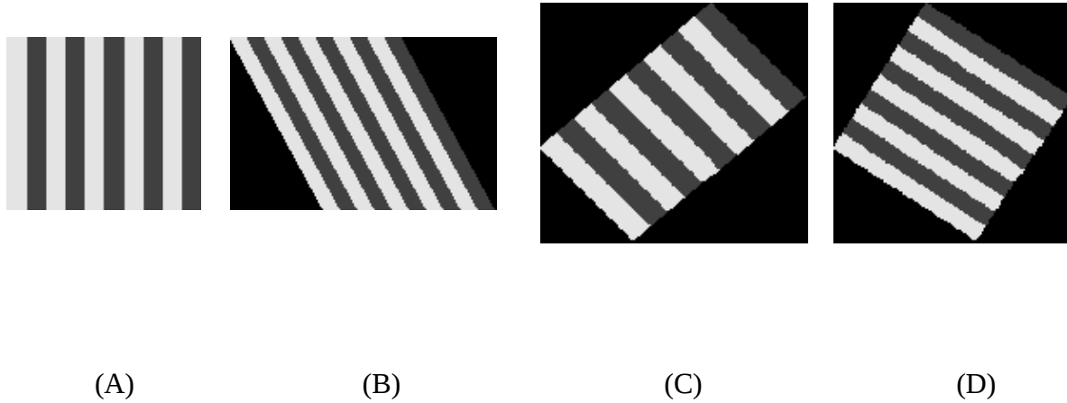
Figure 4: Three-shear rotation of an image counter-clockwise through one radian. The original image (A) is sheared horizontally (B). That image is sheared upwards (C). The final rotated image (D) is on the right.
