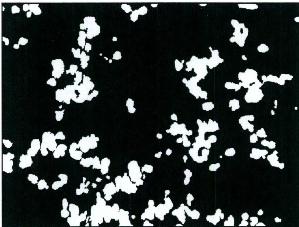
Figure 5. Nickel electrode microstructure used to model cell behavior. The white regions are nickel metal and black regions active material. The image corresponds to a 60 by 40 \mu\text{m} cross-sectional region of the nickel electrode.
